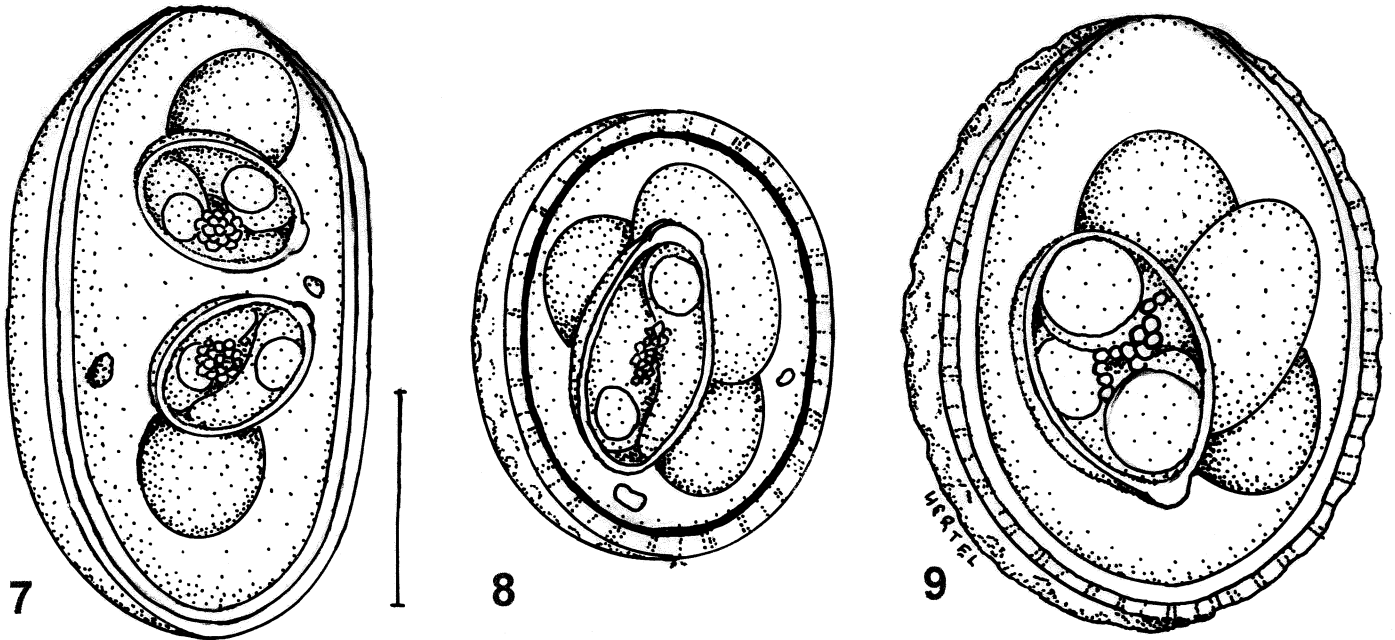
FIGURES 7–9. Line drawings of sporulated oocysts. 7. E. kamoshika . 8. E. serowi . 9. E. crispus . Bar = 10 \mu\text{m} .
