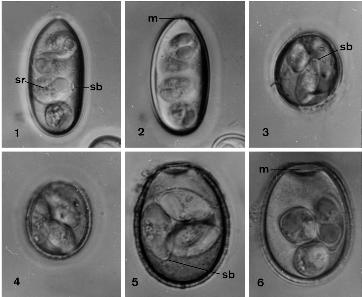
FIGURES 1–6. Photomicrographs of sporulated oocysts of Eimeria kamoshika (1, 2), Eimeria serowi (3, 4), and Eimeria crispus (5, 6) from C. crispus collected on Mt. Zao, Yamagata Prefecture, Honshu, Japan. Bar = 10 \mu m. 1, 2. Note asymmetrical shape of oocyst, presence of an M (but no M cap), sporocyst shape, presence of an SB, and SR. 3, 4. Note mildly striated appearance of oocyst wall(s) in optical cross section, apparent lack of an M, ellipsoidal shape of sporocyst, presence of an SB, and SR. 5, 6. Note thick, striated oocyst wall, presence of a wide M, ellipsoidal shape of sporocyst, presence of an SB, and SR. Abbreviations: m, micropyle of oocyst; sb, Stieda body; sr, sporocyst residuum.
