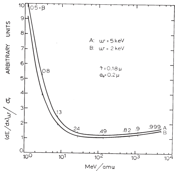
Figure 7. The ratio of two criteria for grain counts: (dE/dx)_{\text{restricted}} (in AgBr) (1) / \sigma_{\tau} (6)
