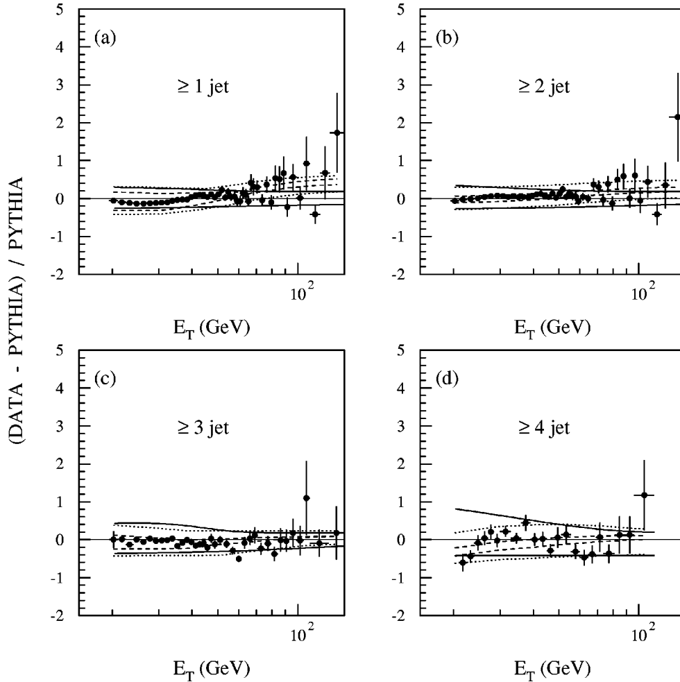
FIG. 2. (\text{Data} - \text{PYTHIA}) / \text{PYTHIA} as a function of the transverse energy of the leading jet for (a) single-jet inclusive, (b) two-jet inclusive, (c) three-jet inclusive, and (d) four-jet inclusive event samples. The relative systematic uncertainties in the cross section corresponding to the energy calibration added in quadrature with 15% uncertainty in luminosity are shown by the solid lines. The uncertainty in the ratio (\text{Data} - \text{MC}) / \text{MC} from energy and angle smearing is shown by the dashed lines. The total uncertainty on the ratio is shown by the dotted lines.
