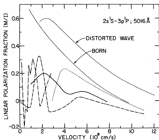
FIG. 11. Linear polarization fraction of the 2s^1S-3p^1P 5016 Å transition vs relative collision velocity. Heavy unbroken line represents current density ( 30 \pm 5 \mu\text{A cm}^{-2} ) foil data. Dashed line, proton impact excitation (Refs. 35–38); dotted line, electron excitation (Refs. 39 and 40) dashed line with dots, electron pickup by fast \text{He}^+ from Ne gas (Ref. 42). First Born and distorted wave calculations are also shown (Refs. 44 and 47).
