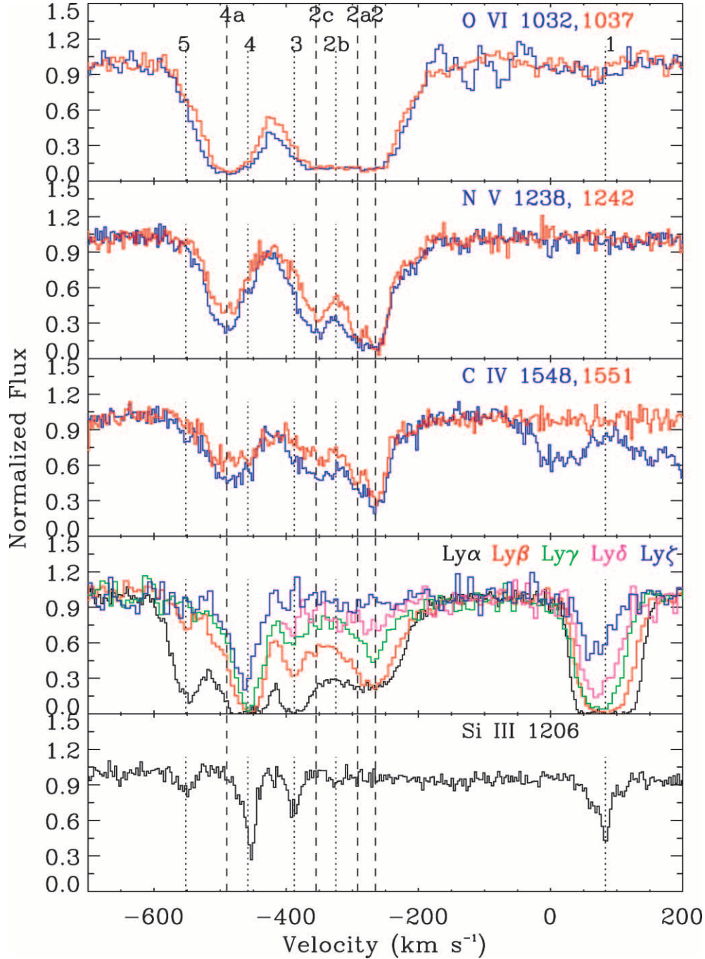
FIG. 2.—Normalized absorption profiles from 2003 May STIS and FUSE spectra. The spectra are plotted as a function of radial velocity with respect to the systemic redshift of the host galaxy. The centroid velocities of kinematic components associated with the AGN outflow are identified with dashed vertical lines. Components identifying low-ionization absorbers likely unrelated to the outflow (see text) are shown with dotted lines. The difference in kinematic structure is evident in comparing the high-ionization CNO doublets with Si III. The Ly \delta profile is not plotted at v < -400 km s ^{-1} because of contamination with Galactic absorption at these velocities.
