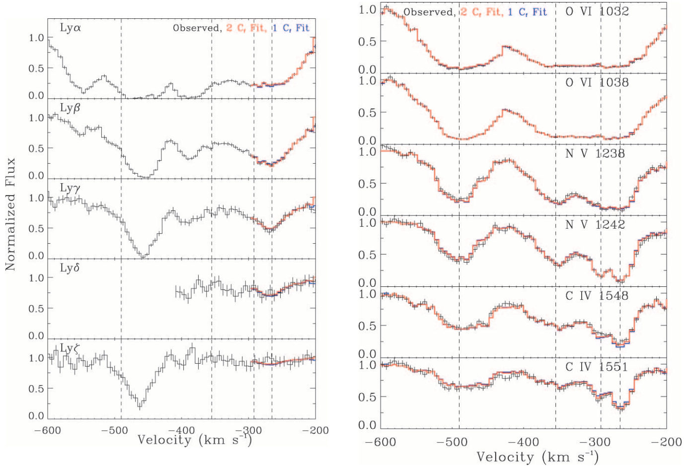
FIG. 6.—Best-fit intrinsic absorption profiles for the Lyman lines ( left ) and CNO doublets ( right ) from the two geometric models. The normalized observed spectrum is plotted in black, model A profiles are in blue, and model B profiles in red. The model profiles were derived from the best-fit covering factors and column densities shown in Figs. 3 and 4 using eq. (4). The contaminated region of the Lyman line fit (Figs. 3 and 4, dotted lines ) is not plotted.
