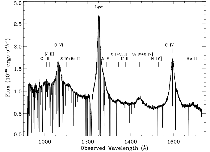
FIG. 1.—Full far-UV spectrum of the active nucleus in Mrk 279 from the FUSE and HST /STIS spectra obtained in 2003 May. Emission lines are labeled above the spectrum. The data were heavily binned for clarity in presentation.
