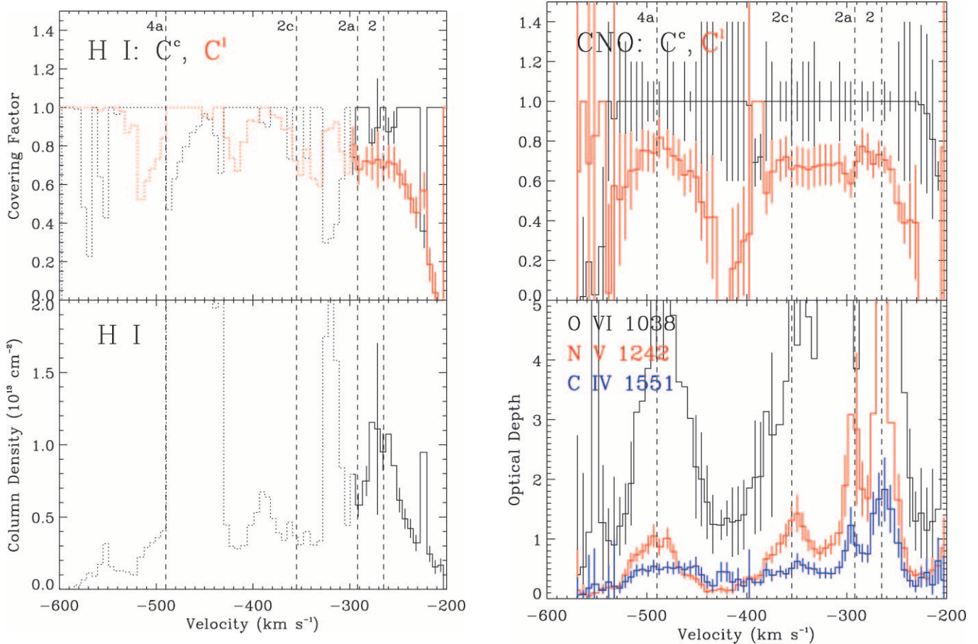
FIG. 5.—Same as Fig. 4, but for the two covering factor geometric model (model B). Continuum covering factors are plotted in black and emission-line covering factors in red.
