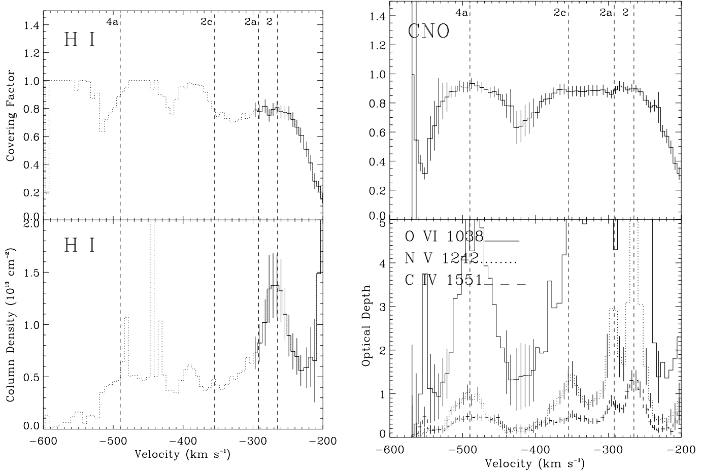
FIG. 4.—Best-fit covering factor and column density/optical depth solutions from \chi^2 minimization for the single covering factor geometric model (model A). Top panels show C solutions, solved independently for the Lyman series (left panels) and combined CNO doublets (right panels). Bottom panels show the H I column density and C IV (dashed histogram), N V (dotted histogram), and O VI (solid histogram) optical depth solutions. The contaminated, and thus unreliable, region of H I absorption is plotted with dotted histograms.
