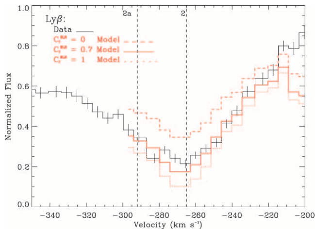
FIG. 10.—Constraints on the covering factor of the high blueshifted velocity O \nu_{\text{BLR}} by the Ly \beta absorber. The observed normalized Ly \beta profile (black) is compared with models derived for three values of emission-line covering factor (red). Models were derived using the observed Ly \gamma absorption, as described in the text. Models with an unocculted (dashed line) and fully occulted (dotted line) BLR are ruled out. An emission-line covering factor of 0.7 (solid line), consistent with the global fits, matches most of the observed profile well.
