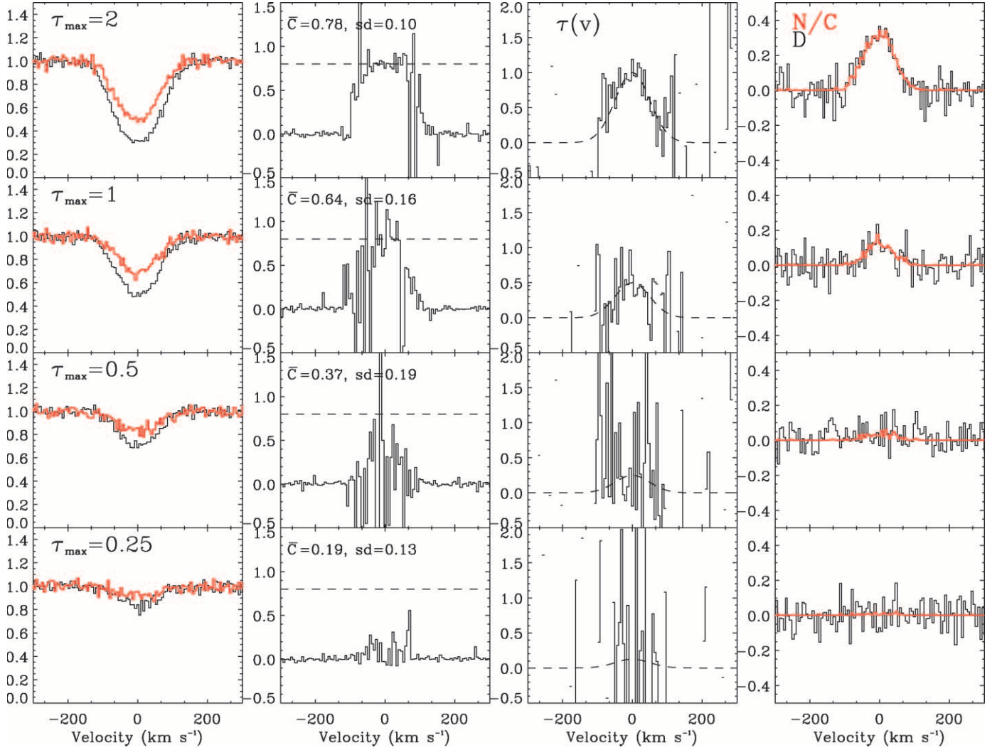
FIG. 11.—Systematic errors in the doublet solution resulting from spectral noise. Left panels show synthetic normalized doublet profiles (long-wavelength members in red) with simulated noise for a range of absorption strengths. The peak \tau in the blue doublet member is given at the top of each panel. The second and third columns show the C and \tau profiles, respectively, derived from the doublet solution (eq. [3]); means and standard deviations (sd) measured for C in the central 150 \text{ km s}^{-1} are printed. The actual constant covering factor, C = 0.8 , and Gaussian \tau profiles are shown with dashed lines for comparison. Right panels show the value of the numerator ( N ) of the doublet equation divided by C (red) and the denominator ( D , black). Because of the nonlinear form of N , N/C drops below the noise level in D for low \tau and thus biases the solution to underestimates of C . The discrepancy increases for weaker absorption.
