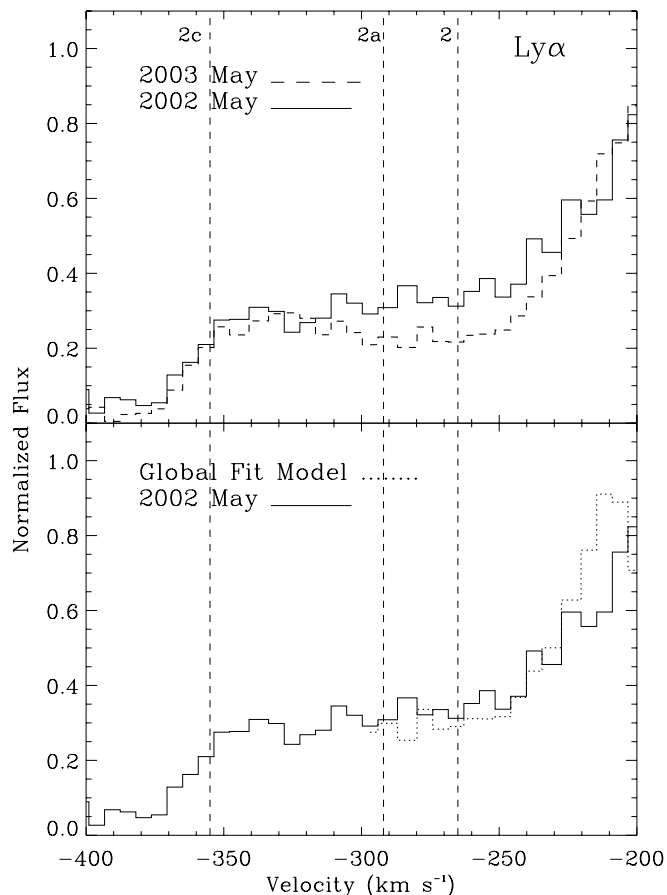
FIG. 8.—Variability in Ly \alpha absorption. The top panel shows that Ly \alpha absorption in components 2–2a was shallower in a 2002 May STIS spectrum ( solid histogram ) than in 2003 May ( dashed histogram ). The bottom panel shows that a model of the 2002 profile ( dotted histogram ), constructed with individual covering factors derived from the 2003 spectrum (Fig. 5), matches the observed profile well. This indicates the variation in absorption depth is likely due to a change in effective covering factor resulting from different relative strengths of the continuum and emission-line fluxes in the two epochs.
