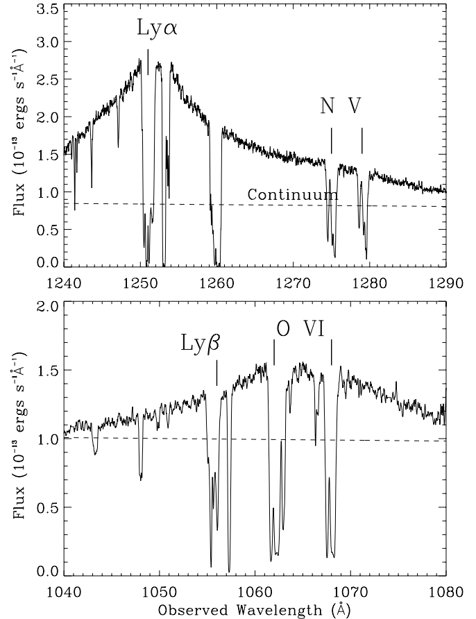
FIG. 3.—Spectrum of Ly \alpha -N v (top) and Ly \beta -O VI (bottom), illustrating complexities in treating covering factors in intrinsic absorption measurements. The continuum flux level, plotted as dashed lines, is essentially identical for each pair of lines, while the emission-line fluxes underlying each line differ greatly. This has important implications for the relative effective covering factors. In addition, the nature of the BLR emission underlying these lines is complex: Ly \beta absorption lies on the high-velocity blue wing of O VI, while N v absorption has a contribution from the red wing of the Ly \alpha BLR.
