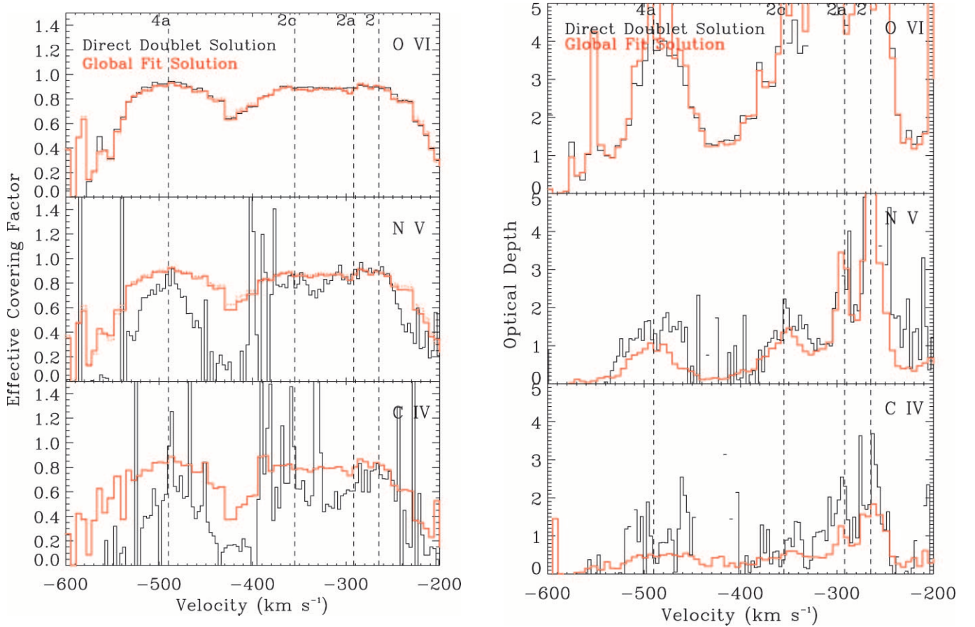
FIG. 9.—Comparison of covering factor and optical depth solutions derived with the global-fitting ( red ) and single-doublet ( black ) methods. Left panels : Covering factors from the global-fitting method are the effective values derived by weighting the individual covering factors in model B by their respective fluxes. The short-wavelength doublet members are plotted with solid red lines and the long-wavelength members with dotted lines. Right panels : Optical depths for the long-wavelength lines of the doublets.
