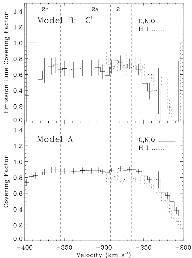
FIG. 7.—Comparison of covering factor solutions for the two independent methods: Lyman and global CNO doublet lines. Top : Best-fit solutions to the emission-line covering factors from model B. Bottom : Single covering factor solutions from model A.
