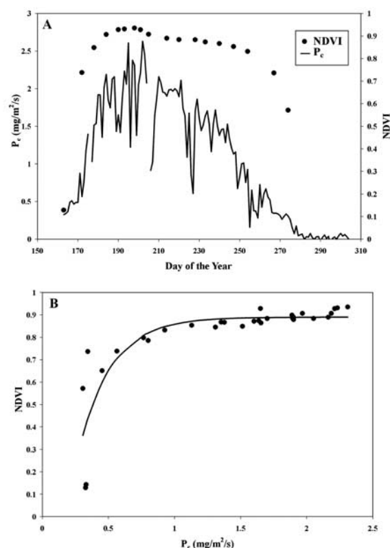
Figure 2. (A) Temporal behavior of NDVI and mid-day canopy photosynthesis ( P_c ) of maize, during the growing season of 2001. (B) Relationship between NDVI and mid-day canopy photosynthesis ( P_c ), established for both study sites.
