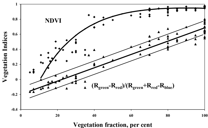
FIGURE 5. NDVI and newly developed vegetation index (R_{\text{green}} - R_{\text{red}}) / (R_{\text{green}} + R_{\text{red}} - R_{\text{blue}}) versus vegetation fraction for wheat canopy
