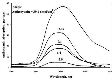
FIGURE 3. Anthocyanin absorption retrieved from absorption spectra of leaves with equal Chl content and different Anth content
