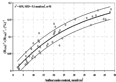
FIGURE 4. Index for anthocyanin estimation plotted versus anthocyanin content
