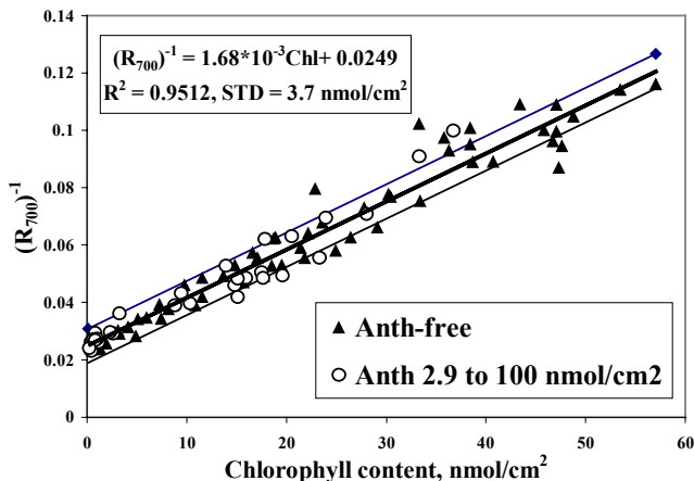
FIGURE 1. Inverse reflectance at 700 nm vs. Chl content for Anth-containing and Anth-free leaves.
