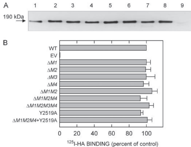
Figure 2. Expression and 125 I-HA ligand binding of 190-HARE CD mutants. Cells were grown to confluence, washed twice with cold PBS, and centrifuged cell lysates (25 μg of protein) were subjected to SDS-PAGE and electrotransfer. A , HARE protein was detected by Western blot analysis using anti-V5 Ab. The 190-HARE proteins are as follows: lane 1, WT; lane 2, ΔM1; lane 3, ΔM2; lane 4, ΔM3; lane 5, ΔM4; lane 6, ΔM1M2; lane 7, ΔM1M2M4; lane 8, Y2519A; and lane 9, EV. B , ligand blot assays were performed with 125 I-HA in multiple experiments using different clones of the indicated mutants, and HARE expression was determined by Western blotting using the same strips after autoradiography. 125 I-HA ligand blot signals were normalized to HARE expression using densitometry and to WT (as 100%).
