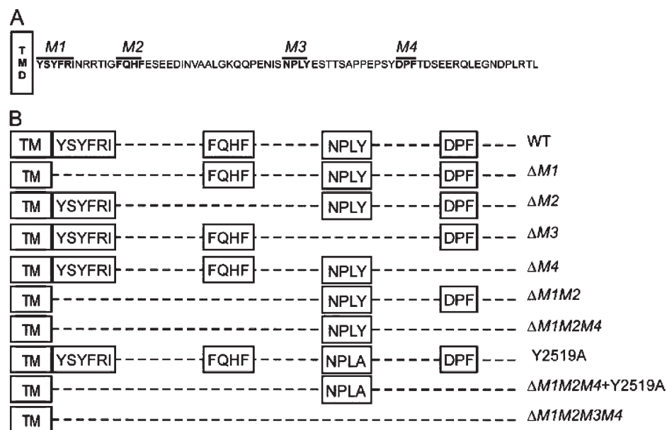
Figure 1. The 190- and 315-HARE CD and mutants used in this study. A , four putative endocytic motifs (indicated in boldface and overlined ) are present in the 72-aa CD of recombinant 190-HARE (1416 aa long) or 315-HARE (2551 aa long). The four sequence motifs (YSYFRI 2485 , FQHF 2495 , NPLY 2519 , and DPF 2534 ) are referred to as M1, M2, M3, and M4, respectively. Numbering is relative to the full-length 315-HARE protein (13, 15). V5 and His 6 epitopes are at the COOH termini of all 190-HARE mutants. B , scheme illustrates the various motif deletion or site-specific 190-HARE CD mutants used. Constructs and stably transfected Flp-In-293 cell lines were prepared as described under "Experimental Procedures." TM, transmembrane.
