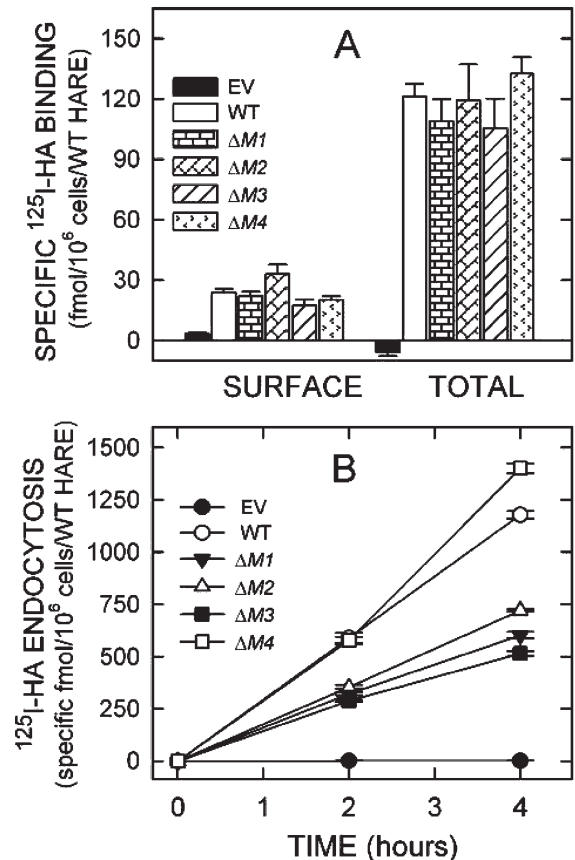
Figure 3. 125 I-HA binding and endocytosis by cells expressing single motif 190-HARE mutants. Cells expressing EV, WT, or mutant 190-HARE were incubated in serum-free medium and washed, and specific 125 I-HA binding at 4 °C or endocytosis at 37 °C was quantified as described under "Experimental Procedures." A , cell surface and total cellular 125 I-HA binding are indicated for cells expressing 190-HARE: WT (white bars), ΔM1 (horizontal rectangles), ΔM2 (diagonal rectangles), ΔM3 (diagonal lines), or ΔM4 (arrowheads) 190-HARE or EV (black). Values from 2 to 3 independent experiments are the means ± S.E. ( n = 6–9) specific 125 I-HA binding normalized for HARE expression relative to WT 190-HARE. B , specific 125 I-HA internalization was determined at 37 °C for 2 and 4 h as described under "Experimental Procedures." Values from 2 to 3 independent experiments are the mean ± S.E. ( n = 6–9) specific 125 I-HA endocytosis, normalized for HARE expression relative to WT. The plots show cells expressing WT (○), ΔM1 (▼), ΔM2 (Δ), ΔM3 (■), or ΔM4 (□) 190-HARE, or EV (•).
