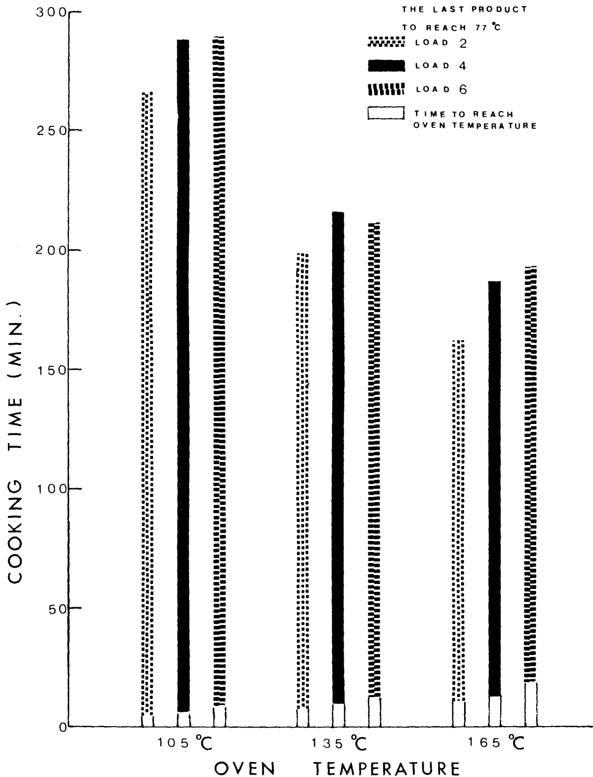
Figure 4. Time Needed to Reach Predetermined Oven Temperatures and Total Cooking Times for All Turkey Rolls to Reach 77°C or above in a Convection Oven When Using Three Oven Loads and Three Oven Temperatures.
