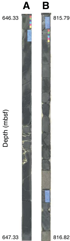
Figure 6. Split-core photos of rocks recovered from (A) 646.33–647.33 mbsf and (B) 815.79–816.82 mbsf.
