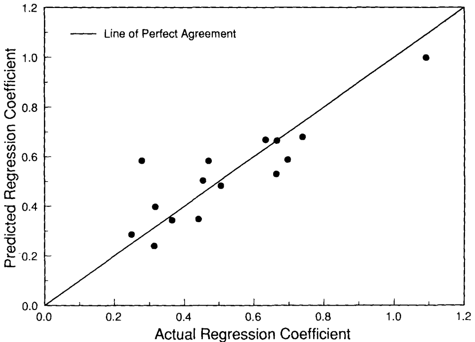
Fig. 13. Predicted vs. actual regression coefficients for estimating interrill sediment delivery rates on non-ridged plots.
