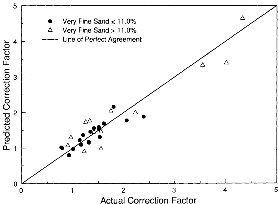
Fig. 9. Predicted vs. actual correction factors for estimating rill sediment delivery rates under rainfall conditions.
