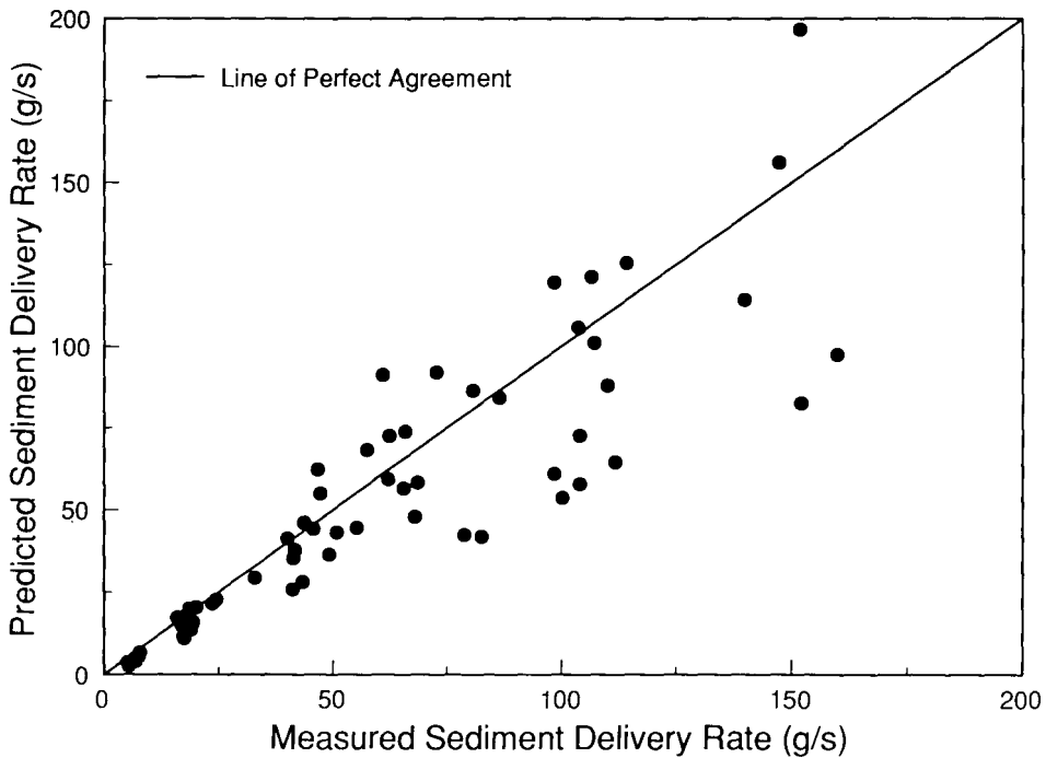
Fig. 4. Predicted vs. measured rill sediment delivery rates with rainfall for a Nansene soil.
