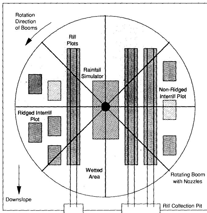
Fig. 1. Plot diagram of a rainfall simulation site.
