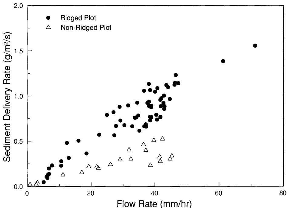
Fig. 10. Interrill sediment delivery rates vs. flow rates for a Nansene soil.
