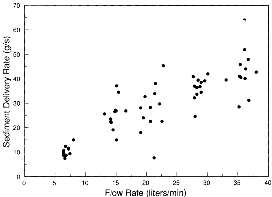
Fig. 6. Rill sediment delivery rates without rainfall vs. flow rates for a Nansene soil.
