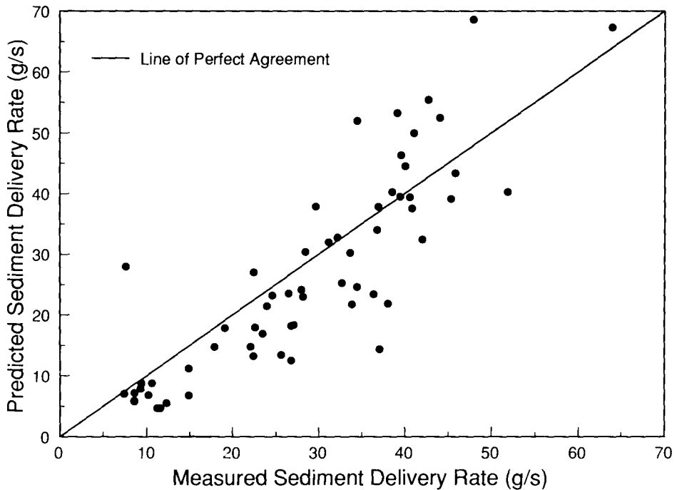
Fig. 7. Predicted vs. measured rill sediment delivery rates without rainfall for a Nansene soil.
