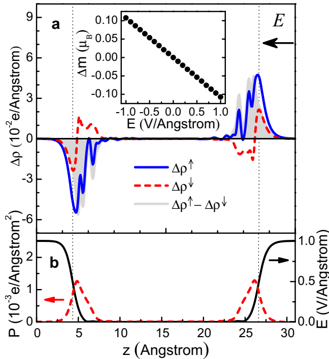
FIG. 3. (Color online) Effects of electric field on electronic properties of a 22-Å-thick \text{CrO}_2 (001) film along the z direction normal to the film surface. (a) Induced spin-dependent charge densities \Delta\rho = \rho(E) - \rho(0) for majority-( \uparrow ) and minority-( \downarrow ) spin electrons and spin density \Delta\rho^\uparrow - \Delta\rho^\downarrow averaged over the film plane per unit cell area A = 19.55 \text{ \AA}^2 . Inset: induced magnetic moment \Delta m per unit cell area of the \text{CrO}_2 (001) surface as a function of the applied electric field. (b) Variation in the electric field (solid line) and the induced minority-spin polarization (dashed line) across the film. The applied external electric field is E = 1.0 \text{ V/\AA} , pointing from right to left. The vertical lines show schematically the two surfaces of the \text{CrO}_2 film.
