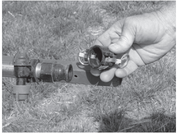
Figure 7. End cap on wet boom to drain and flush boom.
