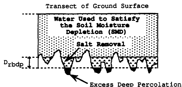
FIG. 5. Deficit Irrigation Nonbeneficial DP
