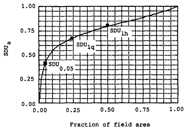
FIG. 13. Relationship between SDU_a and Defining Fraction of Field Area Having Lowest Depths in Distribution (Values Normally Distributed with CV = 0.25 )
