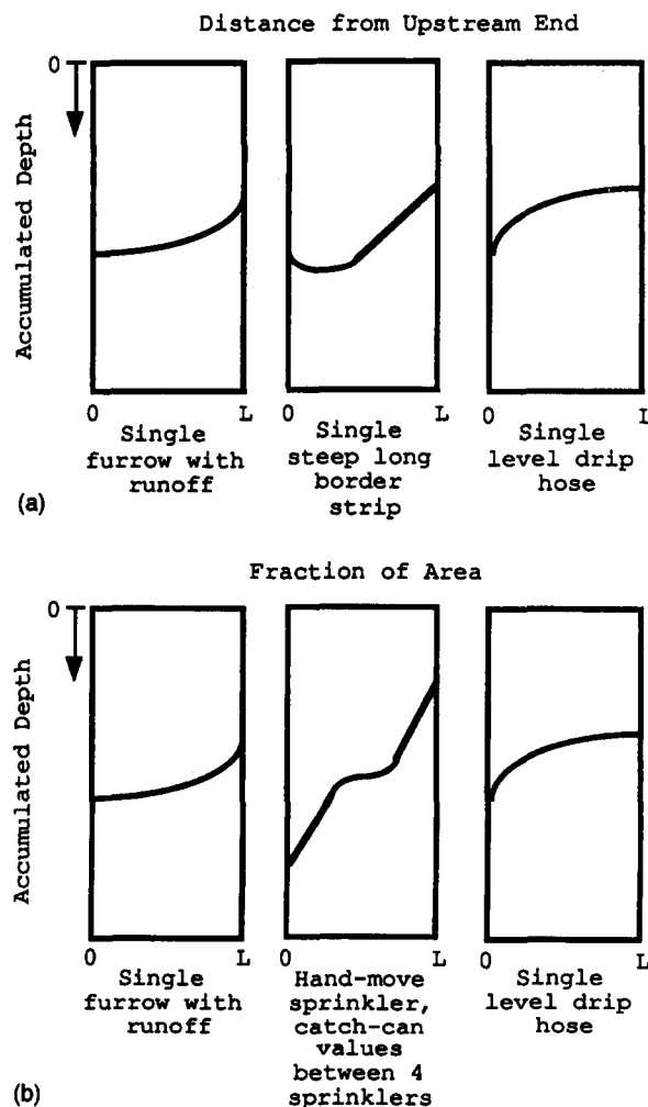
FIG. 12. Typical Variations in Accumulated Water with Location and Arranged by Magnitude: (a) Typical Variation in Local Accumulation of water; Furrow and Border Strip Variations due to Opportunity-Time Differences Only; Drip Variation due to Pressure Variation Only; (b) Typical Variation in Water Accumulated; Values Are Arranged by Magnitude, Rather Than by Location
