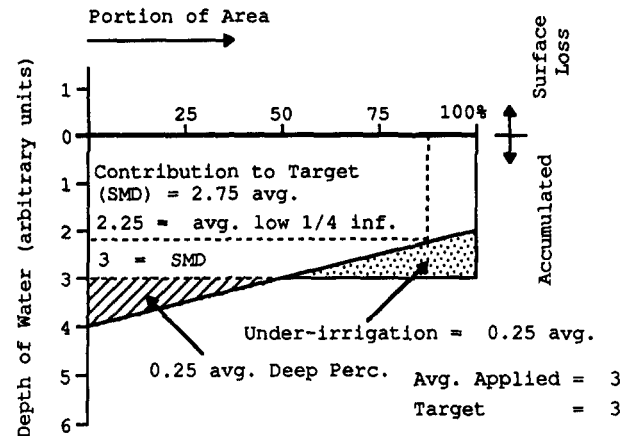
FIG. 15. Water Destination Diagram with Average Accumulated Depth Equal to Target Depth (3 Units) and No Surface Losses: DU_{iq} = 2.25/3 = 0.75 ; AD_{iq} = 0.75 (Underirrigation)
