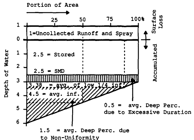
FIG. 16. Overirrigation on All of Field: DU_{iq} = 3.38/4.5 = 0.75 ; AE = 2.5/5.5 \times 100 = 45.5\% ; AD_{iq} = 3.38/3 = 1.13 > 1.0 (Overirrigation)
