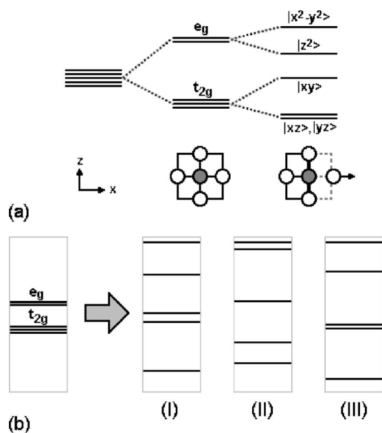
FIG. 4. Crystal-field splitting for 3d ions (dark) coordinated by oxygen atoms (white). Weak deviations from cubic symmetry (a) leave the levels reminiscent of the cubic e_g-t_{2g} splitting, whereas strong deviations (b) yield a complete remixture of the levels. The cases (I)–(III) are typical splittings at low-indexed surfaces, each corresponding to a different atomic environment.
