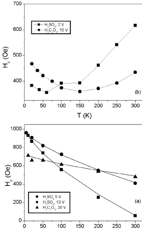
Figure 2. H_c as a function of T as measured by a SQUID for Ni nanowires anodized in (a) H 2 SO 4 at 5 V (No. 1) and 10 V (No. 2) and H 2 C 2 O 4 at 20 V (No. 3); the solid curves are fitting curves and (b) H 2 SO 4 at 2 V (No. 4) and H 2 C 2 O 4 at 10 V (No. 5).
