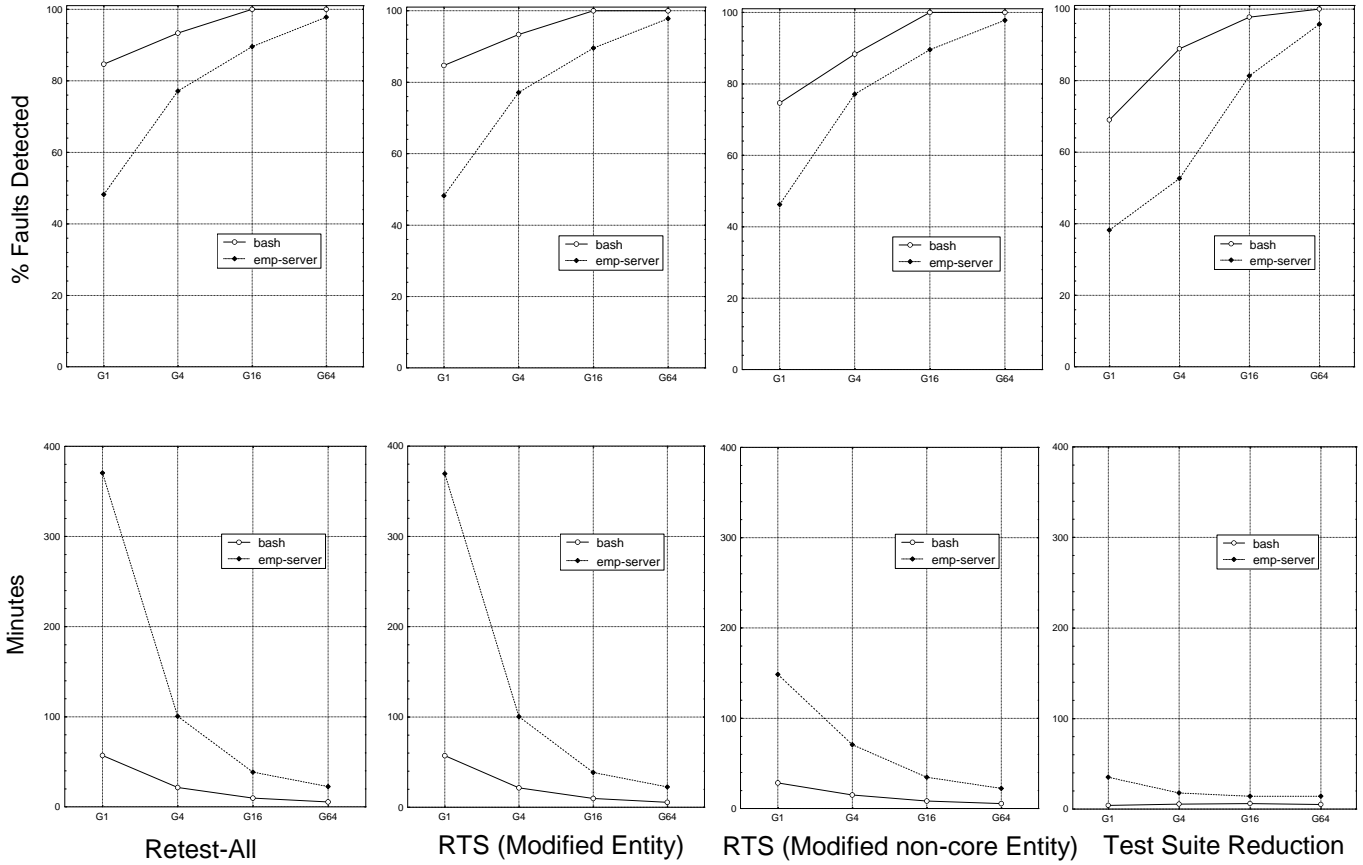
Figure 1: Fault detection effectiveness (top) and test execution time (bottom) for regression test selection and test suite reduction techniques across test suite granularities, averaged across versions.
