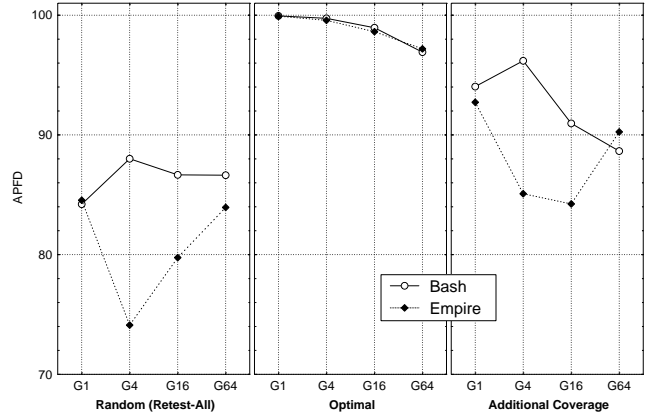
Figure 2: APFD for test case prioritization.
