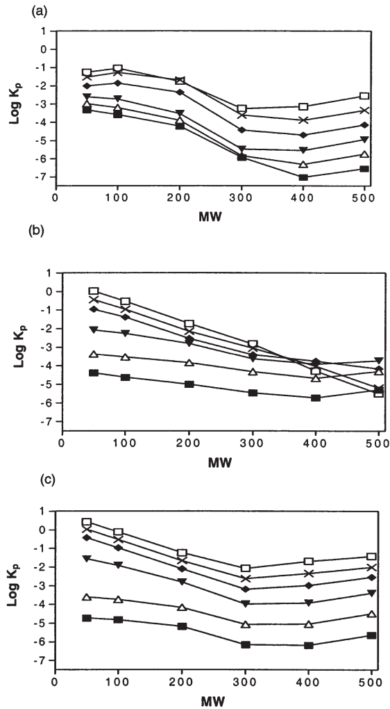
Figure 4. Effect of molecular weight on Log K_p at (a) 25 °C, (b) 32 °C, and (c) 37 °C. Data are divided by log K_{ow} : -1(■), 0 (◆), 1 (△), 2 (▼), 3 (×), and 4 (□).
