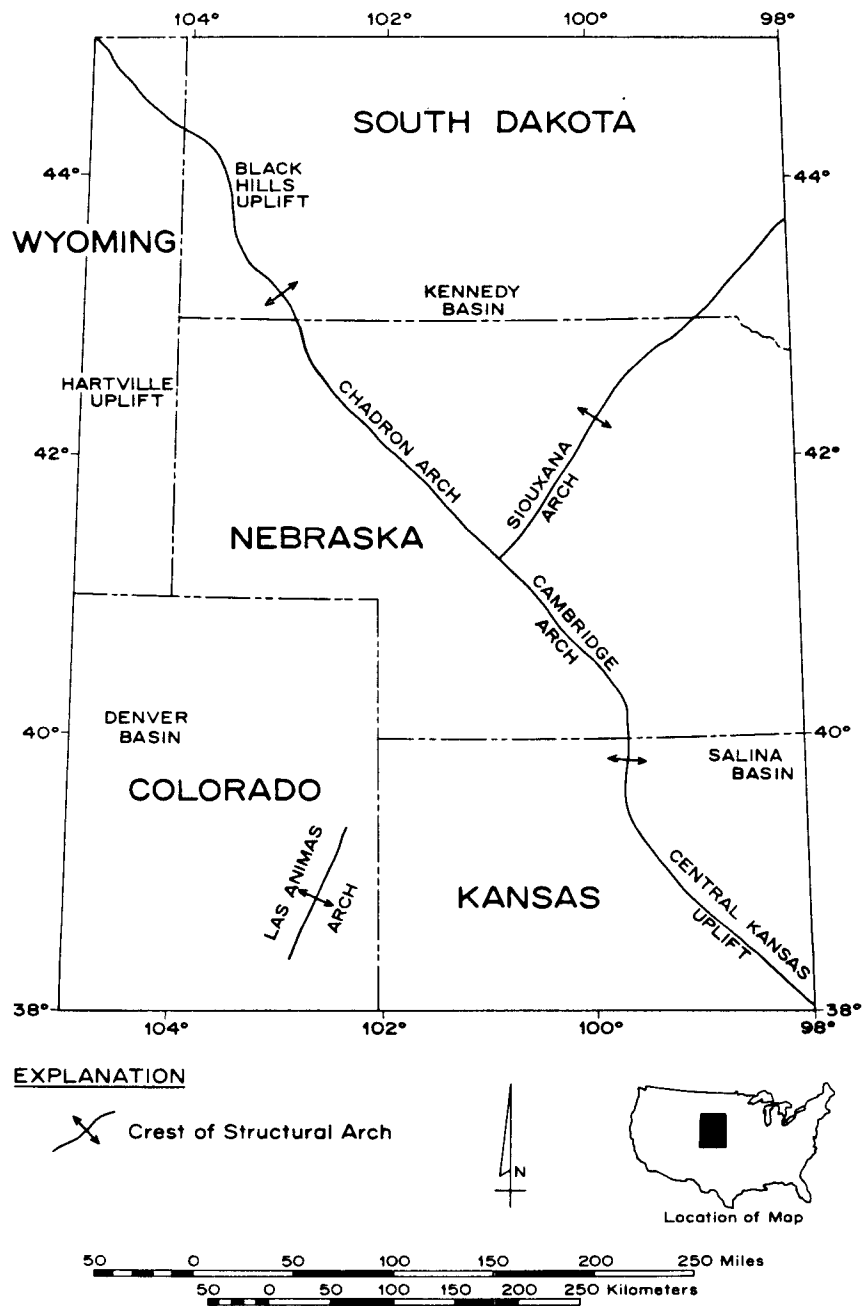
Fig. 1. Major tectonic elements of the central Cordilleran foreland (modified from Bayley and Muehlberger 1968).
