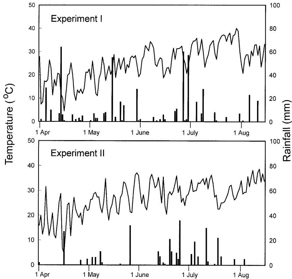
Fig. 1. Daily high temperature ( ^{\circ}\text{C} ; lines) and precipitation (mm; solid bars) at the University of Nebraska-Lincoln Havelock Agronomy Farm in 1999 (Exp. I) and 2000 (Exp. II) (High Plains Regional Climate Center, 2000).
