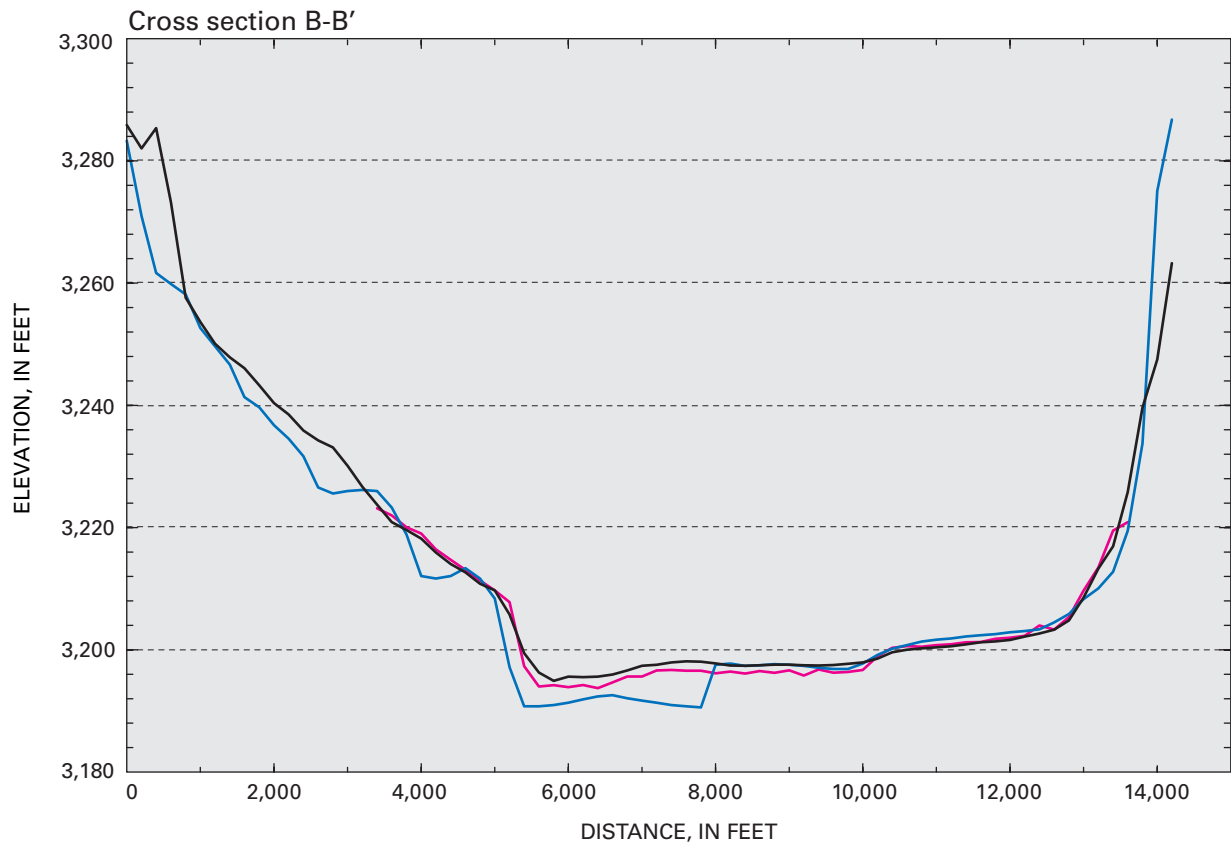
Figure 9. Selected cross sectional profiles of the lake showing dual-frequency data, Lake McConaughy, Nebraska.
