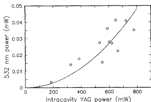
FIG. 3. The peak SHG power vs the peak fundamental intracavity power in a 1.3-mm-thick crystal. The line is a least-squares fit to the relationship P_{2\omega} = S(P_\omega)^2 with S = 8 \times 10^{-5} \text{ W/W}^2 .
