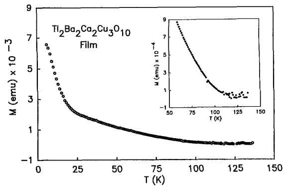
Fig. 7 Flux trapping versus temperature for the film annealed at 895°C for 1 hour. This data were obtained after cooling in the applied field of 50 kOe, removing the field and taking the data on warming in zero field.
