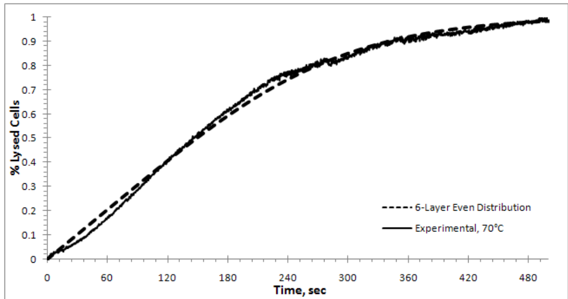
Figure 4.9: A comparison of the multi-layer model result (— — —) with initial data that corresponds to an even distribution over 6 layers and the experimental curve (————) at 70^\circ\text{C} . The best fit is obtained for k = 0.0205 \text{ s}^{-1} .
