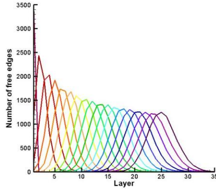
Figure 4.5: Progression of the pdf (not normalized) through cell wall layers, generated by the Monte Carlo method for a two-dimensional model that measures N \times M = 3500 \times 35 .
