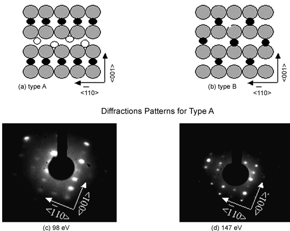
Figure 8. A schematic of the \text{Co}_3\text{O}_4(110) two ideal bulk termination structures: (a) type A and (b) type B, and the LEED data indicating type A termination taken at (c) 98 eV and (d) 147 eV incident electron beam energies. The LEED were acquired at 300 K.
