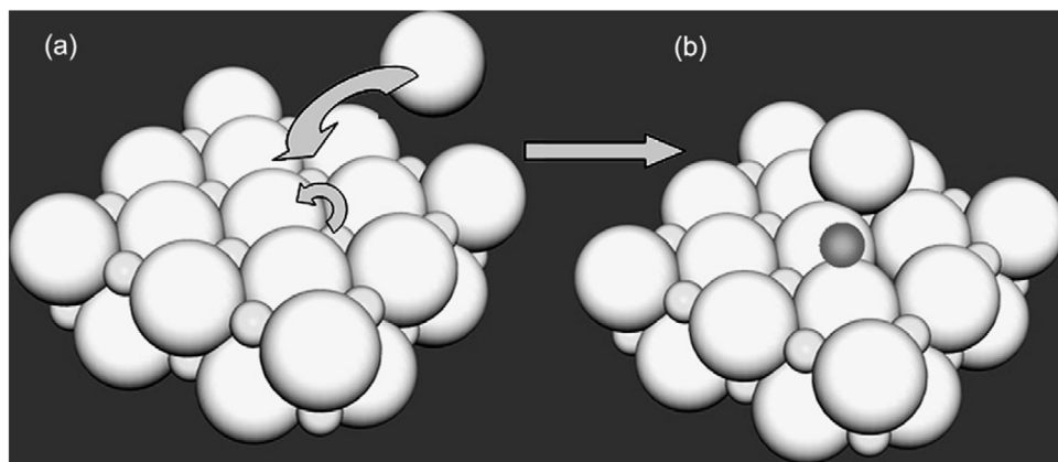
Figure 2. Schematic diagram illustrating the ease with which a cation in an octahedral site of a rocksalt lattice can move to a tetrahedral sites at the surface.
