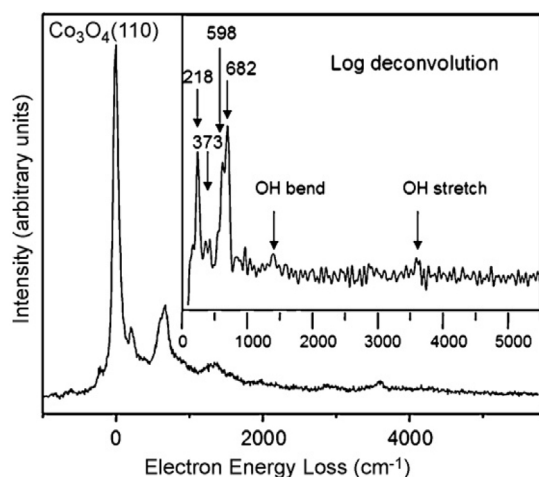
Figure 10. HREELS spectrum of UHV-conditioned (sputter/anneal) \text{Co}_3\text{O}_4(1\ 1\ 0) with the inset showing deconvolution to reveal four well-developed phonon modes at 218, 373, 598 and 682 \text{cm}^{-1} . Data were acquired with a primary energy beam of 3.77 eV.
