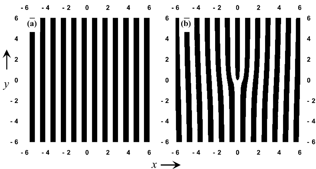
Fig. 2. Computer-generated binary patterns based on Eq. (1), for K = 2\pi . Each pattern consists of 1000 \times 1000 pixels, with pixels for which T=0 rendered black and T=1 , white. Pattern (a) has no encoded vortex ( M=0 in Eq. (1)). Pattern (b) has a single fringe bifurcation ( M=1 ); when used as a hologram it gives rise to vortices with topological charge \pm 1 in the \pm first diffraction order.
