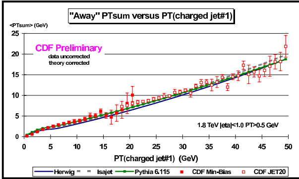
Figure 31. Data from Fig. 26 on the average scalar p_T sum of charged particles ( p_T > 0.5 \text{ GeV} and |\eta| < 1 ) as a function of p_T(\text{jet\#1}) (leading charged jet) for the “away” region defined in Fig. 24 compared with the QCD “hard scattering” Monte-Carlo predictions of HERWIG 5.9, ISAJET 7.32, and PYTHIA 6.115. The errors on the (uncorrected) data include both statistical and correlated systematic uncertainties. The theory curves are corrected for the track finding efficiency and have an error (statistical plus systematic) of around 5%.
