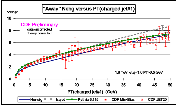
Figure 30. Data from Fig. 25 on the average number of charged particles ( p_T > 0.5 \text{ GeV} and |\eta| < 1 ) as a function of p_T(\text{jet\#1}) (leading charged jet) for the “away” region defined in Fig. 24 compared with the QCD “hard scattering” Monte-Carlo predictions of HERWIG 5.9, ISAJET 7.32, and PYTHIA 6.115. The errors on the (uncorrected) data include both statistical and correlated systematic uncertainties. The theory curves are corrected for the track finding efficiency and have an error (statistical plus systematic) of around 5%.
