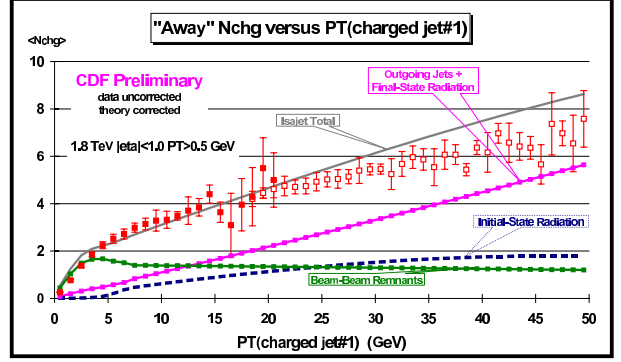
Figure 32. Data from Fig. 25 on the average number of charged particles ( p_T > 0.5 \text{ GeV} and |\eta| < 1 ) as a function of p_T(\text{jet\#1}) (leading charged jet) for the “away” region defined in Fig. 24 compared with the QCD “hard scattering” Monte-Carlo predictions of ISAJET 7.32. The predictions of ISAJET are divided into three categories: charged particles that arise from the break-up of the beam and target (beam-beam remnants), charged particles that arise from initial-state radiation, and charged particles that result from the outgoing jets plus final-state radiation (see Fig. 19). The errors on the (uncorrected) data include both statistical and correlated systematic uncertainties. The theory curves are corrected for the track finding efficiency and have an error (statistical plus systematic) of around 5%.
