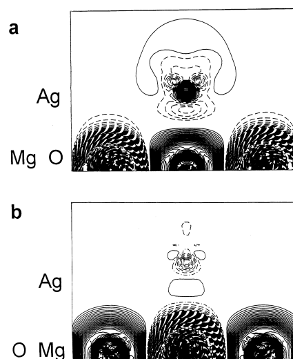
Fig. 4. The difference electronic density maps (the total density minus superposition of atomic densities) or the cross-section perpendicular to the (100) interface plane for \frac{1}{4} Ag adsorption: (a) over O and (b) over Mg ions. Isodensity curves are drawn from -1 to +1e a_0^{-3} with an increment of 0.0015e a_0^{-3} . The full, dashed and chained curves show positive, negative and zero difference densities respectively. Note that Ag atoms are strongly polarized: above O ions (a) the electron density is shifted in the direction outwards from the surface, whereas above Mg (b) it is shifted towards surface Mg ions.
