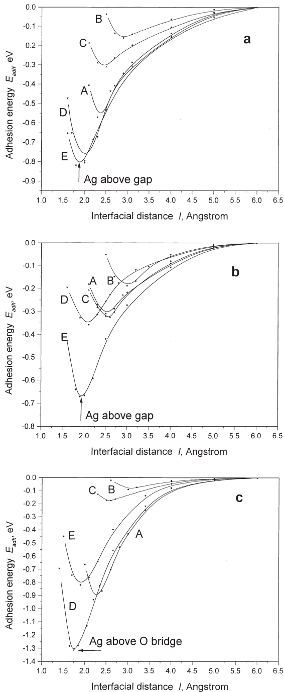
Fig. 5. The interfacial energies for different adsorption sites of Ag atoms on the perfect MgO(110) surface as a function of the distances l between adsorbent and adsorbate (Fig. 2). Three different substrate coverages: half-layer (a), monolayer (b) and bilayer (c) are studied. Full lines are drawn using the standard b-spline option. See notations of the adsorption positions in Fig. 2.
