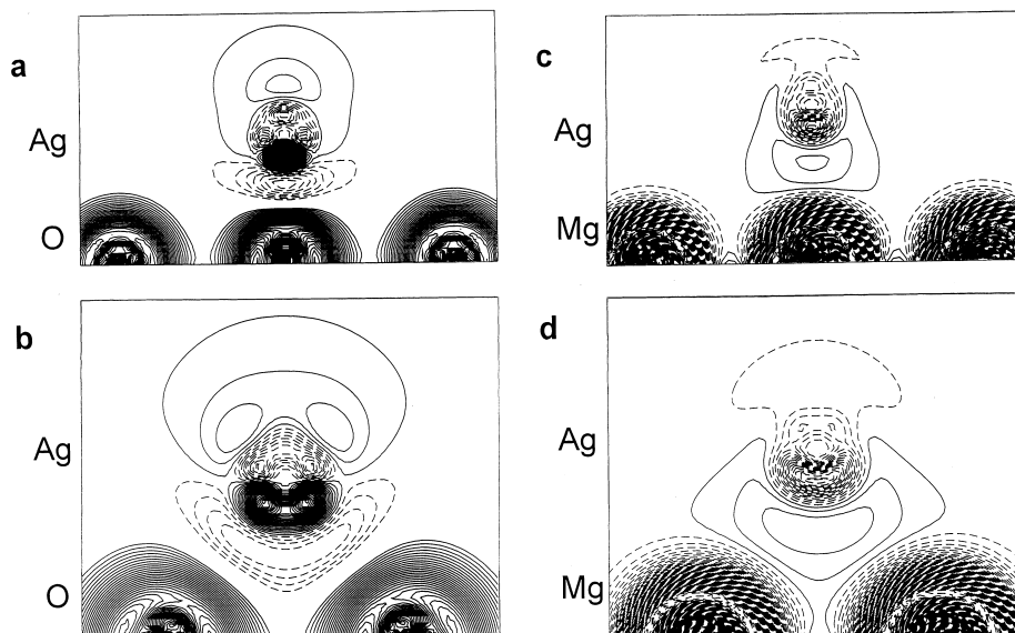
Fig. 6. The difference electronic density maps for the cross-section perpendicular to the (110) interface plane for \frac{1}{4} Ag adsorption: (a) over a single O ion, (b) over O bridge, (c) over a single Mg ion, and (d) over Mg bridge position. Isodensity curves are drawn from -1 to +1e a_0^{-3} with an increment of 0.0015e a_0^{-3} . The full, dashed and chained curves show positive, negative and zero difference densities respectively. As in Fig. 4, Ag atoms are strongly polarized: above O ions (a,b) the electron density is shifted in the direction outwards from the surface, whereas above Mg (c,d) it is shifted towards surface Mg ions. Note that the electron density for O ions (a,b) is visibly compressed in the Ag directions, compared with the other cases shown.
