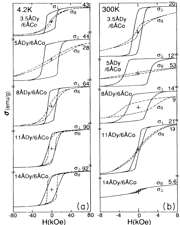
FIG. 10. Hysteresis loops for (Y \text{ \AA} \text{ Dy})/(6 \text{ \AA} \text{ Co}) at 300 \text{ K} and 4.2 \text{ K} .
