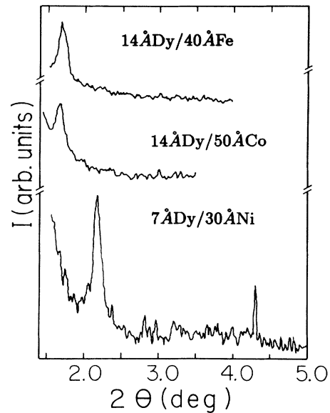
FIG. 2. \text{Cu } K_{\alpha} small-angle diffraction intensity as a function of 2\theta for three Dy/Co, Dy/Fe, and Dy/Ni samples.
