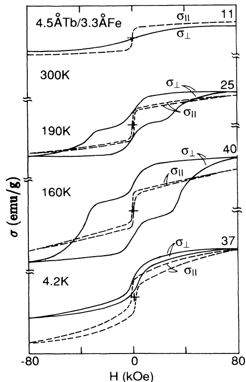
FIG. 23. Temperature dependence of hysteresis loops for (4.5 \text{ \AA Tb})/(3.3 \text{ \AA Fe}) ( X = 300, 190, 160, 4.2 \text{ K} ).
