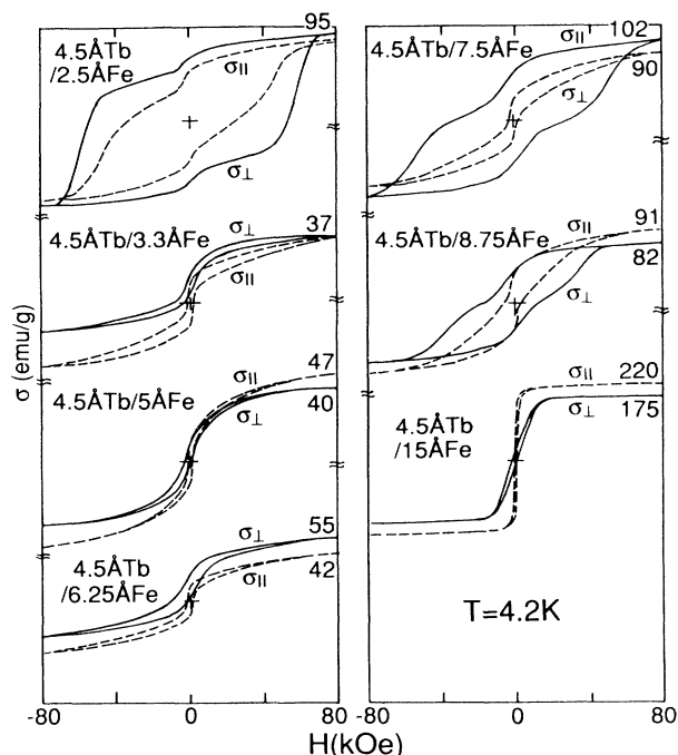
FIG. 22. Hysteresis loops for (4.5 \text{ \AA Tb})/(X \text{ \AA Fe}) ( X = 2.5, 3.3, 5, 6.25, 7.5, 8.75, \text{ and } 15 ) at 4.2 K.
