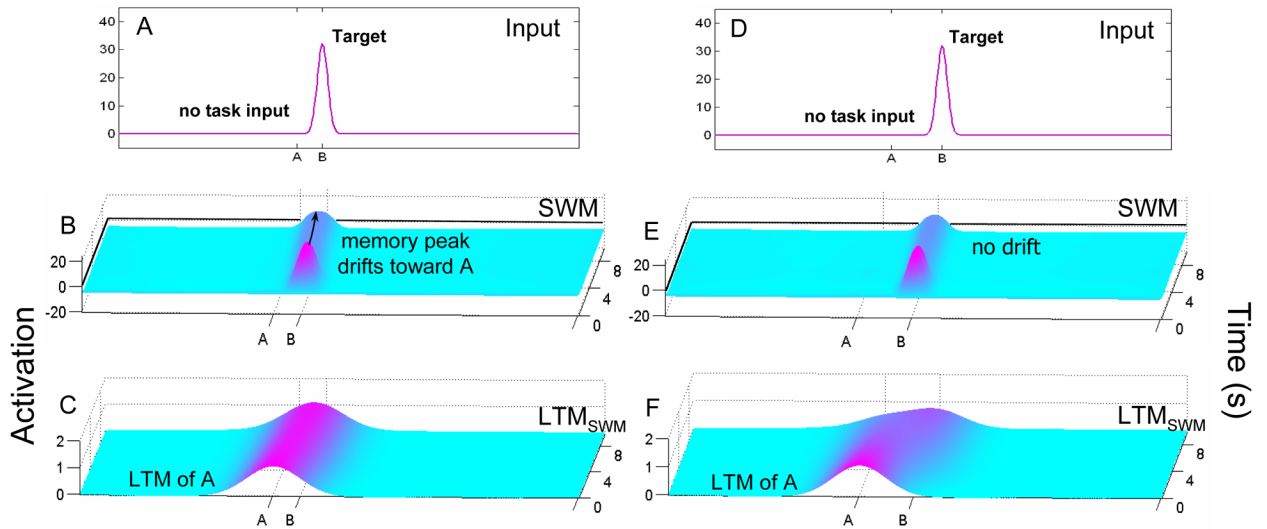
Fig. 4. Simulations of the sandbox A-not-B task. Both simulations began with four trials to the A location with identical inputs (not shown). On the first B trial, the target was presented either near (A-C) or far (D-F) from A. When B was near A (see A), the peak in SWM (B) drifted toward the activation from LTM_{SWM} (C). When B was far from A (see D), on the other hand, the peak in SWM remained stable and did not drift (E). Axes are as in Fig. 1.
