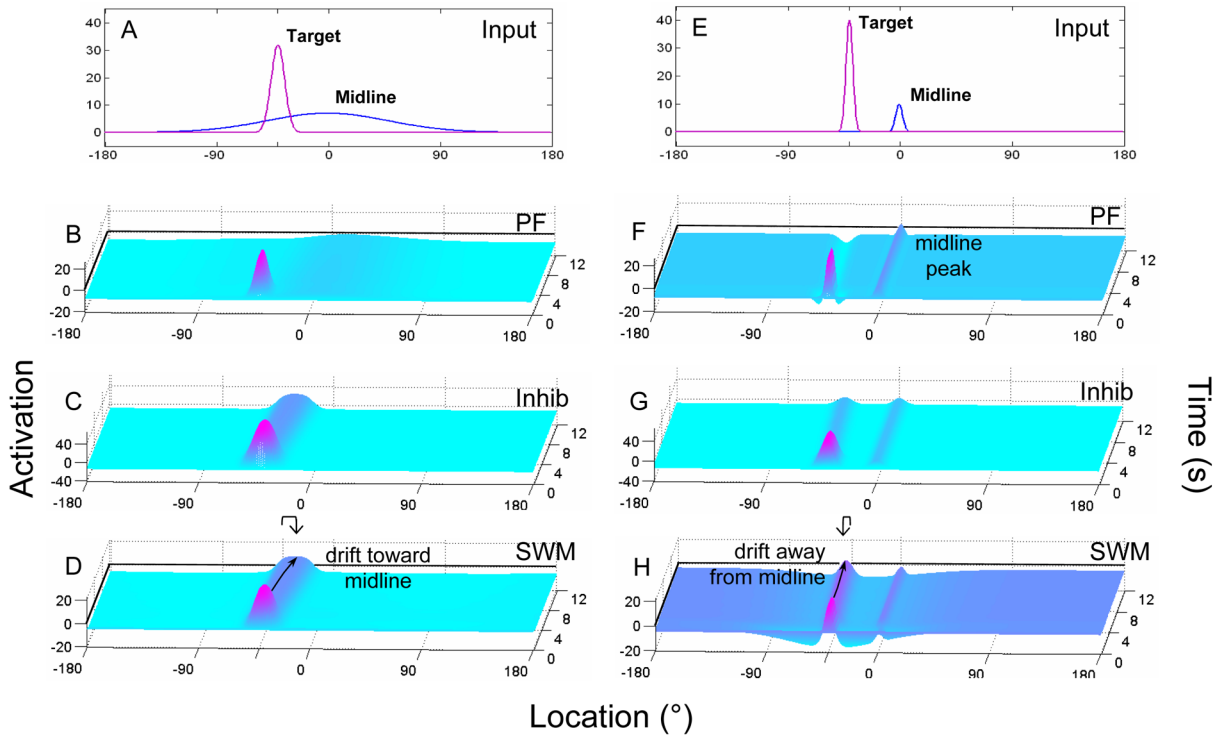
Fig. 5. Simulations of spatial recall trials with child (A-D) and adult (E-H) parameter settings. To approximate developmental changes in reference frame calibration, the inputs are broader and weaker in the child model (A) relative to the adult model (E). In the child model, midline does not provide enough focused input to form a peak in PF (B), and the target peak in SWM (D) is attracted toward the sub-thresholds activation from midline. In the adult model, on the other hand, midline forms a peak in PF (F), which contributes inhibition via Inhib (G) to SWM (H), resulting in the peak being repelled from midline. Axes are as in Fig. 1.
