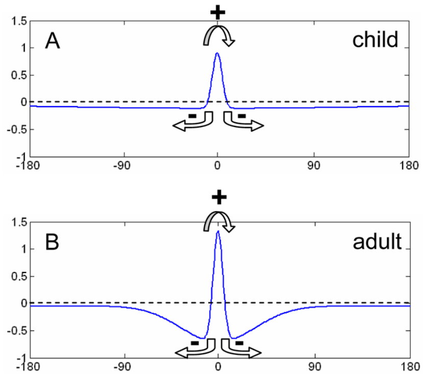
Fig. 2. The local excitation (+) / lateral inhibition (-) function used for child (A) and adult (B) simulations. Dashed line indicates the zero threshold.
