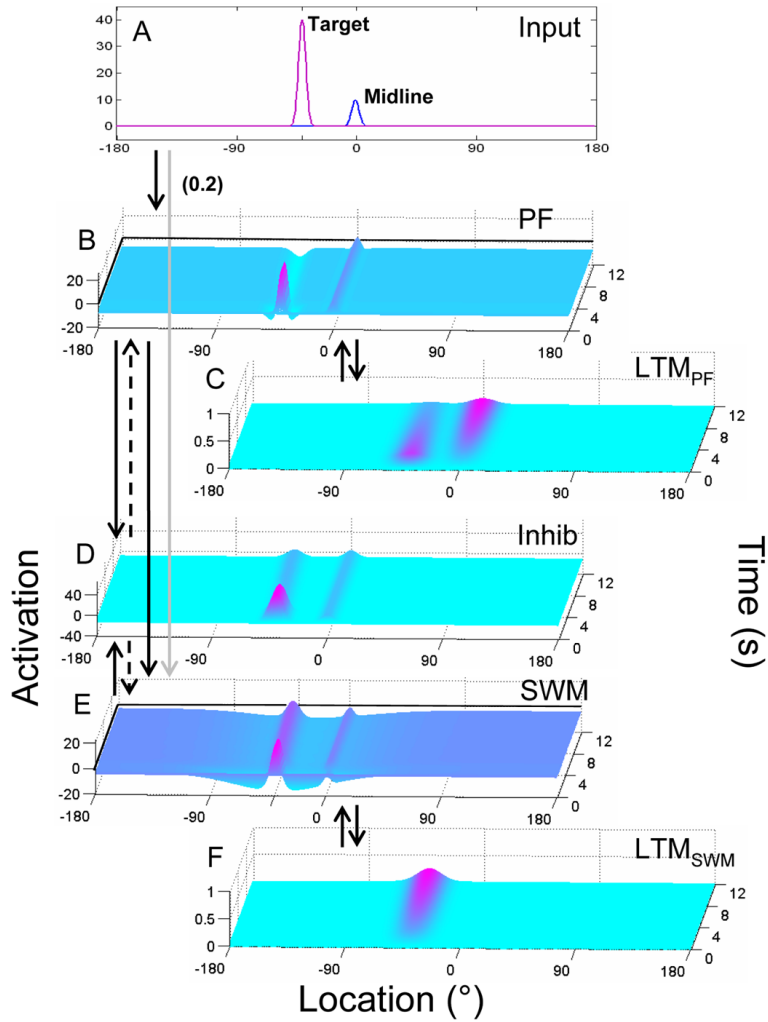
Fig. 1. A simulation of the dynamic field theory performing one spatial recall trial. In each panel, location is across the x-axis, activation on the y-axis, and time on the z-axis. (A) Inputs to the model are presented directly to the model already in an object-centered reference frame (see text for details of the calibration process that transforms spatial information from an egocentric frame of reference in the full model). After this shift, activation is passed to the model consisting of 5 layers: (B) a perceptual field; (C) a long-term memory field associated with this perceptual field; (D) a shared layer of (inhibitory) interneurons; (E) a spatial working memory field; (F) a long-term memory field associated with the spatial working memory field. Solid arrows show excitatory connections between layers, and dashed arrows show inhibitory connections between layers.
