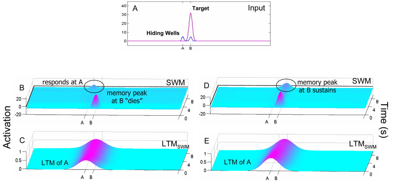
Fig. 3. Simulations of the infant A-not-B task. Both simulations began with four trials to the A location (not shown), then used identical input (A) on the first B trial. Note that these simulations include only the relevant layers of the model, SWM (B, D) and LTM SWM (C, E). Local excitatory interactions were lowest for the “young” infant simulations (B-C), which showed an A-not-B error (see peak circled in B). Local excitation was increased for the “older” infant simulation (D-E), which correctly responded at B (see peak circled in D). Axes are as in Fig. 1.
