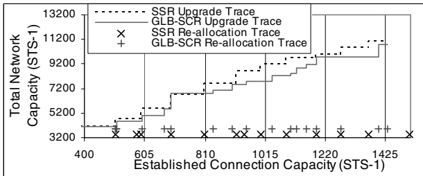
Fig. 9 Upgrade trace and reallocation trace for the non-uniform network when IC=48 and UC=96
