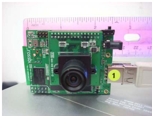
Fig. 1. The wireless embedded smart camera platform employed in the presented system.
