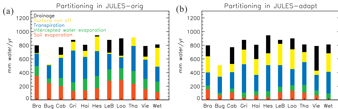
Fig. 3. Simulated mean yearly moisture flux partitioning of total precipitation at the different FLUXNET sites with JULES-orig (a) and with JULES-adapt (b).
