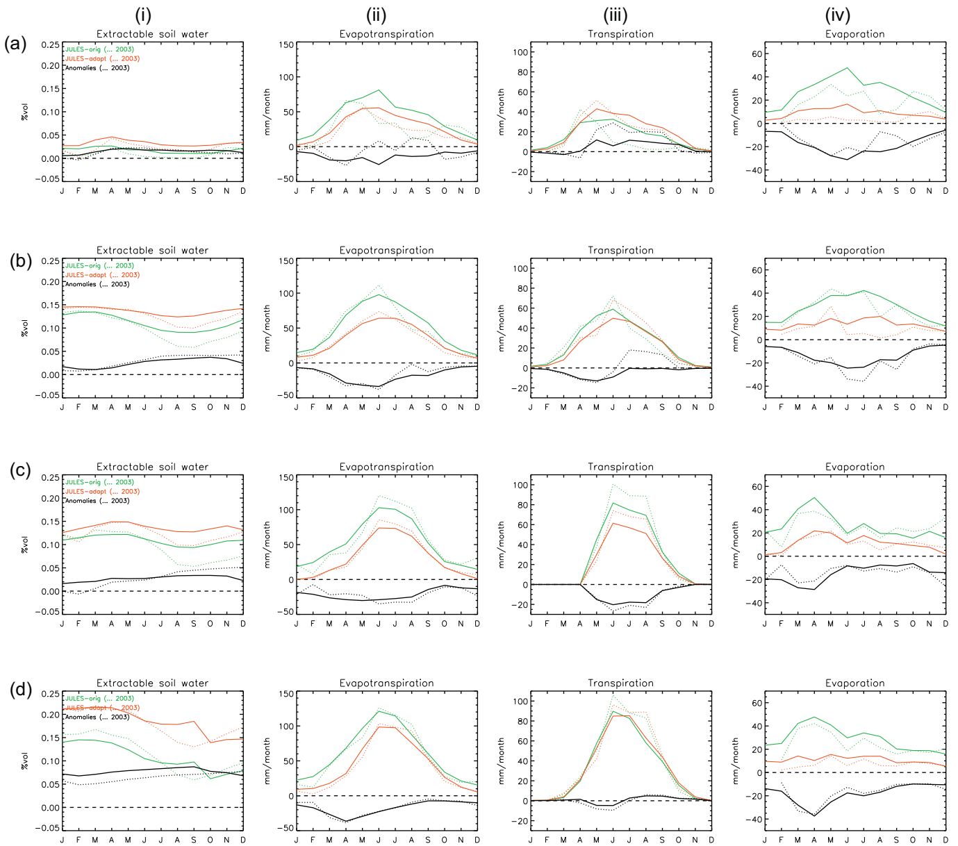
Fig. A.1. The seasonal cycle of the volumetric extractable soil moisture within 3 m depth (i), ET (ii), E_t (iii) and E_s + E_c (iv) simulated over the entire time series with JULES-orig in green and with JULES-adapt in red, with the values for 2003 as dotted lines for Bug (a), Cab (b), Hai (c) and Hes (d). The anomalies between JULES-adapt and JULES-orig are in plain black lines for the entire time series and by dotted black lines for 2003. (For interpretation of the references to colour in this figure legend, the reader is referred to the web version of the article.)
