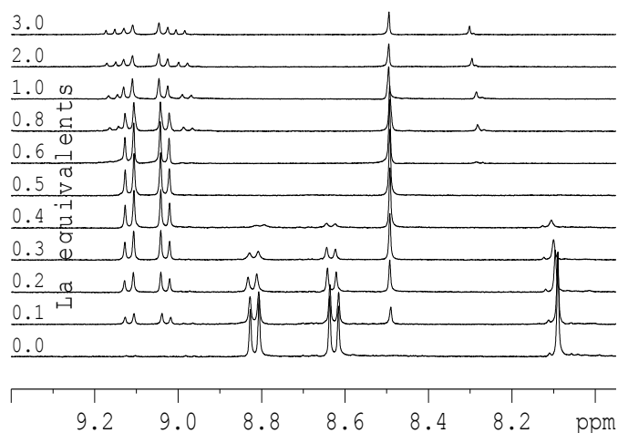
Figure 1.1. Stacked 1 H NMR spectra (8.0-9.3 ppm) of C5-BTPhen titrated with La(NO 3 ) 3 ·6H 2 O in CD 3 CN.
