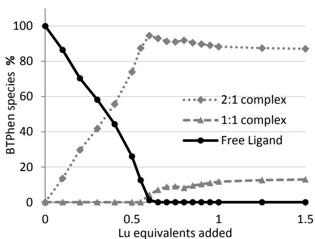
Figure 2.2. Graph showing C5-BTPhen composition at increasing Lu equivalents.
