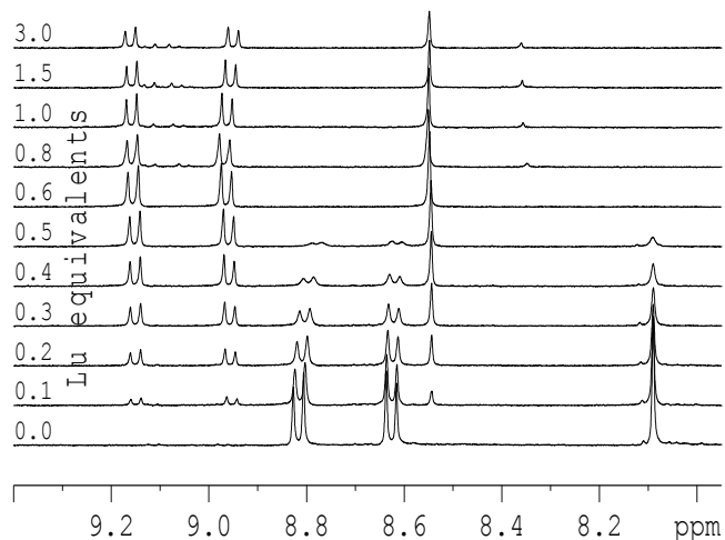
Figure 2.1. Stacked 1 H NMR spectra (8.0-9.3 ppm) of C5-BTPhen titrated with Lu(NO 3 ) 3 in CD 3 CN.
