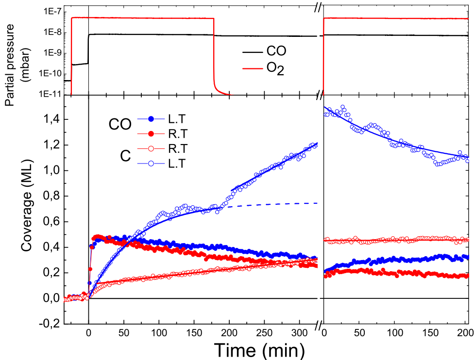
FIG. 2: Left panel: the lower part represents time evolution of the CO (filled symbols) and C (open symbols) XPS peak intensities (with photon energy 630 eV). The measured peak areas were normalized such that the CO saturation coverage at room temperature corresponds to 0.5 ML. The figure shows corresponding experiments at room temperature (red symbols) and at liquid nitrogen temperature (blue symbols). The upper part shows mass spectrometer measurements of the partial pressures at liquid nitrogen temperature. A CO partial pressure of 0.9 \times 10^{-8} mbar range is introduced in the chamber at t=0\text{s} . 15 min after, O 2 partial pressure of 4.9 \times 10^{-8} mbar has been introduced. In both experiments the surface is exposed to CO and O 2 with a partial pressure ratio P(\text{O}_2)/P(\text{CO})=5 . After 285 minutes the O 2 partial pressure is switched off. Right panel: contaminated surface resulting from the previous experiment are exposed again to a mixture of CO and O 2 with a partial pressure ratio P(\text{O}_2)/P(\text{CO})=5 .
