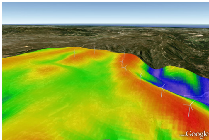
Figure 1. Map of the annual wind power production over a hilly site produced with WAsP
