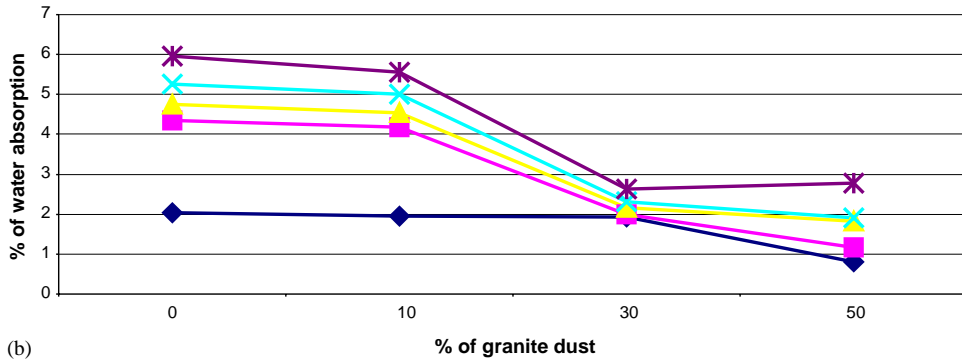
Fig. 5. (a) Graph of %water absorption (1:4); (b) graph of %water absorption (1:3).
