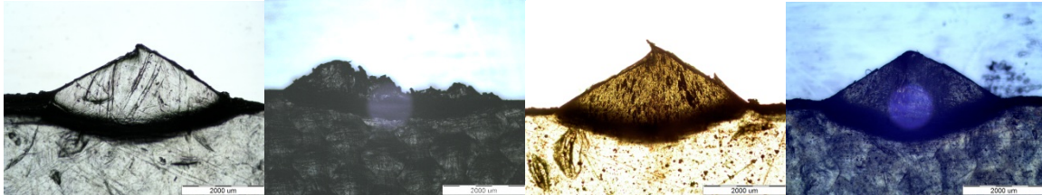
Figure 8. LM pictures taken from the failed DEN-T specimens of the neat PETG, and its nanocomposites containing GR, BA and MMT, respectively (from left to right)
