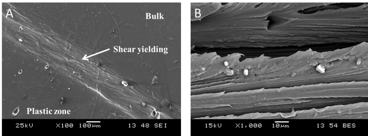
Figure 9. SEM pictures from the surface of the transition between the plastic zone and bulk (A) and from the fracture zone (B) of a DEN-T specimen of PETG-BA
