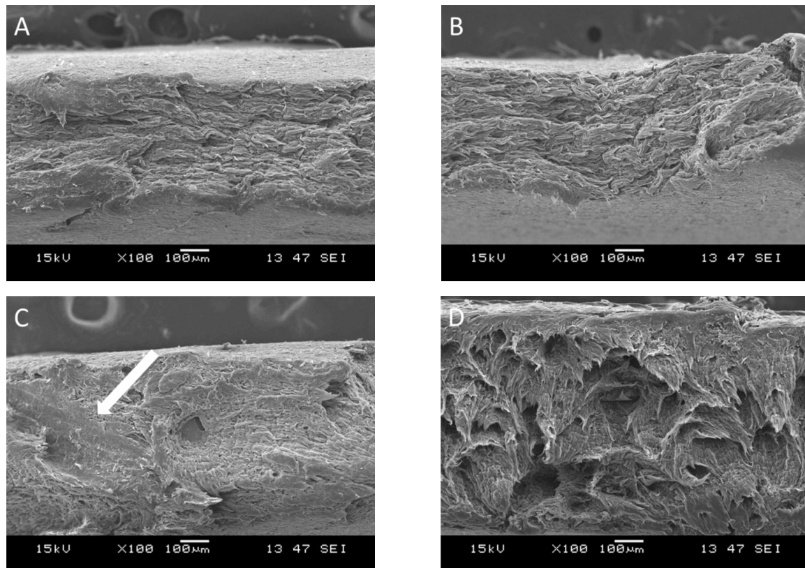
Figure 10. SEM pictures from the fracture zones of DEN-T specimens of EPBC-BA (A), EPBC-MMT (B), EPBC-GR (C) and EPBC-MWCNT (D). Note: secondary cracking is indicated by arrows.
