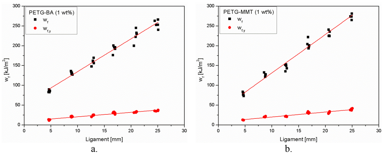
Figure 5. w_f -L traces as a function of the ligament length (L) measured on DEN-T specimens of PETG-BA (a) and PETG-MMT (b)
