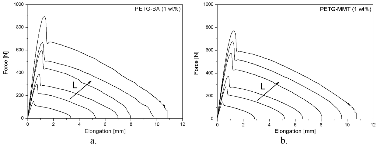
Figure 4. F-x traces as a function of the ligament length (L) measured on DEN-T specimens of PETG-BA (a) and PETG-MMT nanocomposites (b)
