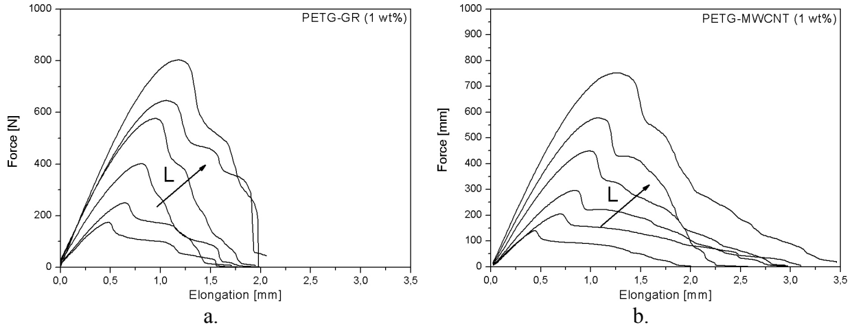
Figure 2. F-x traces as a function of the ligament length (L) measured on DEN-T specimens of PETG-GR (a) and PETG-MWCNT (b). Partitioning between yielding- and necking/tearing-related sections are indicated for the highest ligament specimen
