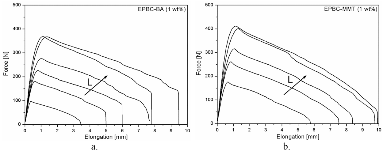
Figure 6. F-x traces as a function of the ligament length ( L ) measured on DEN-T specimens of EPBC-BA (a) and EPBC-MMT nanocomposites (b).
