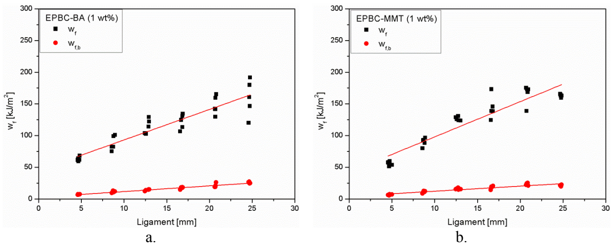
Figure 7. w_f - L traces as a function of the ligament length ( L ) measured on DEN-T specimens of EPBC-BA (a) and EPBC-MMT (b). Note: w_{f,b} is the blunting-related specific work of fracture calculated by considering the absorbed energy until the maximum load.
