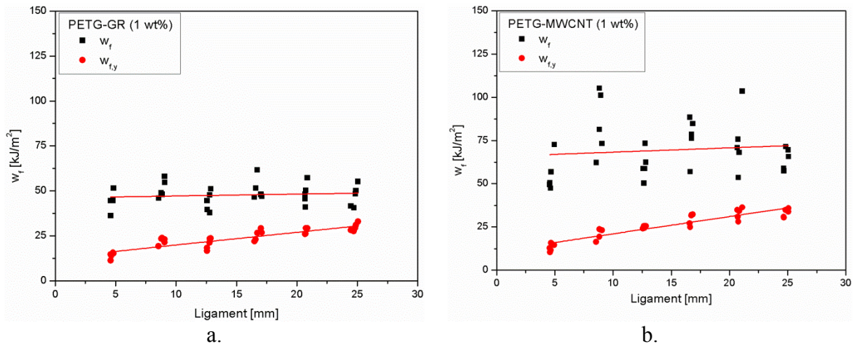
Figure 3. w_f -L traces as a function of the ligament length (L) measured on DEN-T specimens of PETG-GR (a) and PETG-MWCNT (b)
