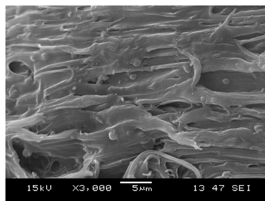
Figure 11. SEM picture from the fracture zone of EPBC-BA
