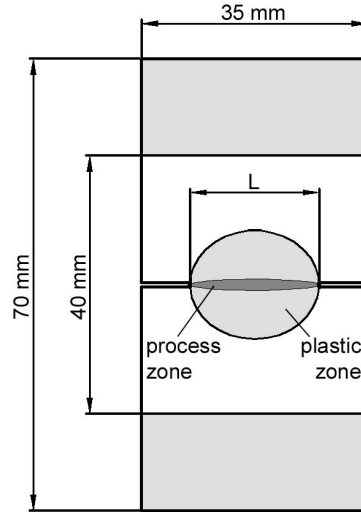
Figure 1. Schematic diagram showing the fracture zones in a DEN-T specimen
