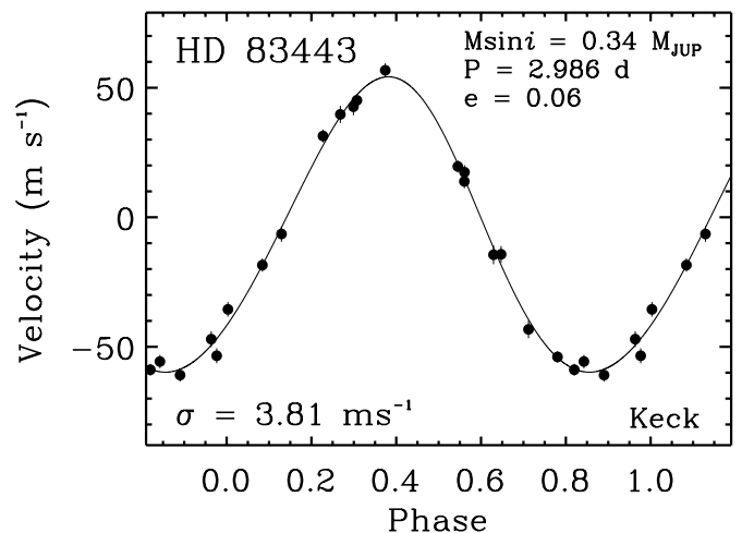
FIG. 1.—Phased Doppler velocities for HD 83443 from Keck. The solid line is the best-fit Keplerian orbit assuming only a single planet. The period p = 2.986 days and semiamplitude K = 57 \text{ m s}^{-1} are nearly identical to the CORALIE parameters for the inner planet. The small rms of the residuals of 3.8 \text{ m s}^{-1} is consistent with errors, implying no evidence for a second planet.
