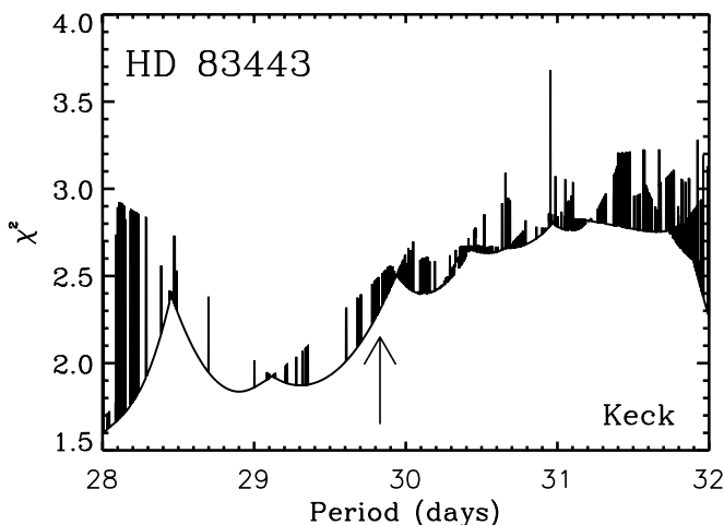
FIG. 7.—Reduced \chi^2 as a function of outer-planet period for a two-Keplerian fit to the Keck data. The period, eccentricity, and amplitude of the inner planet have been frozen at the CORALIE values, as have the eccentricity and amplitude of the outer planet. No minimum is seen in the reduced \chi^2 near 29.83 days, the purported period of the outer planet.
