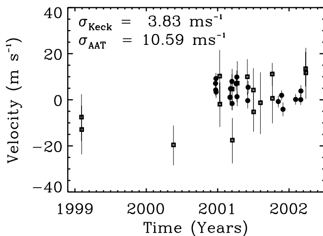
FIG. 4.—Residual velocities from the best-fit single Keplerian for HD 83443, using the combined Keck (circles) and AAT (squares) data. The Keck residuals have an rms of 3.8 \text{ m s}^{-1} , consistent with the combined effects of measurement uncertainty and Doppler jitter. The AAT residuals have an rms of 10.6 \text{ m s}^{-1} , consistent with measurement uncertainty and jitter.
