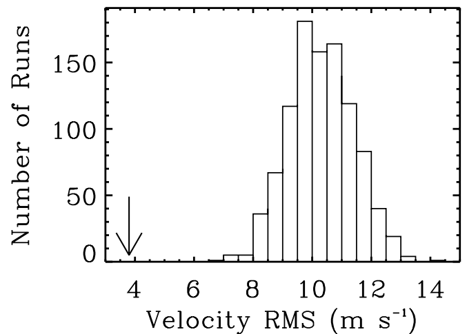
FIG. 6.—Histogram of the rms of the residuals of a single-Keplerian fit to synthetic velocities that stem from a double-planet system. One thousand synthetic Doppler velocity sets were constructed and sampled at the times of the Keck observations, including Gaussian noise. The rms of the residuals to these fits ranges from 6.7 to 14.0 \text{ m s}^{-1} , with a median of 10.3 \text{ m s}^{-1} , well above our errors of 3 \text{ m s}^{-1} . Thus, a single-Keplerian model should fail to adequately fit the double-planet system that was reported. In contrast, the rms of the single Keplerian fitted to the actual Keck data yields an rms of only 3.8 \text{ m s}^{-1} , consistent with noise, indicated by the arrow, suggesting that the second planet does not exist.
