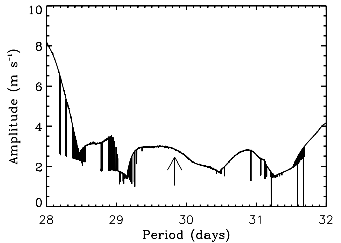
FIG. 8.—Best-fit semiamplitude for the outer planet in a double-Keplerian fit to the Keck data. The period, eccentricity, and amplitude of the inner planet have been frozen at the values reported by CORALIE, as well as the eccentricity of the outer planet. The Keck data rule out an outer planet with a semiamplitude greater than 3 \text{ m s}^{-1} for periods between 29 and 31 days.
