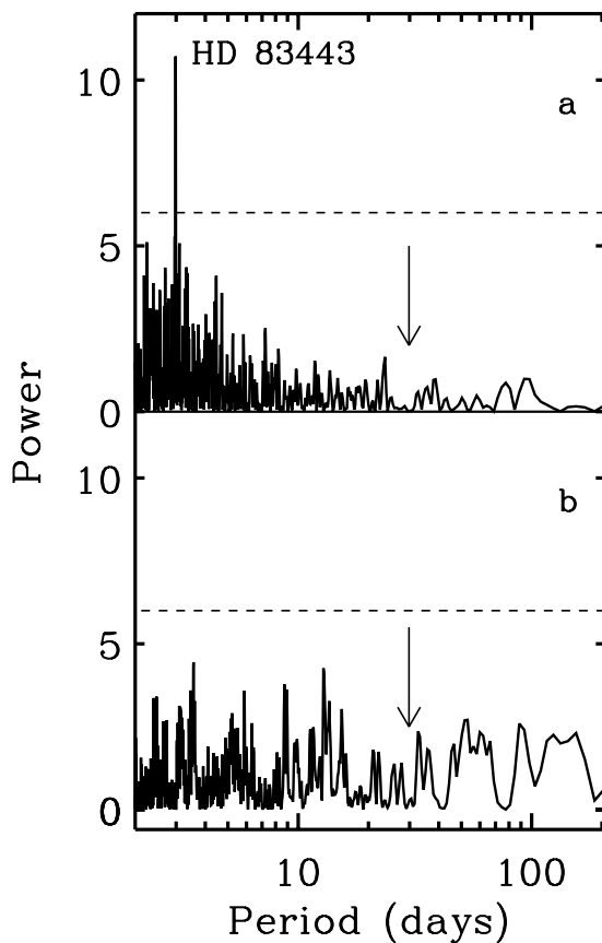
FIG. 5.—Periodogram of HD 83443 Keck velocities. (a) Periodogram of measured velocities. The 2.986 day periodicity is indicated by the highest periodogram peak. The 1% false alarm level is indicated with the dotted line. (b) Periodogram of residual velocities, after subtracting off the best-fit Keplerian. No significant periodicities remain after subtracting off the best-fit single Keplerian. The arrows indicate 29.83 days, the purported period of the outer planet from the CORALIE data.
