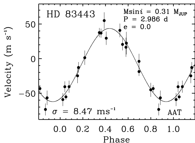
FIG. 2.—Phased Doppler velocities for HD 83443 from the AAT data. The solid line is the best-fit Keplerian orbit assuming only a single planet. The period p = 2.986 days and semiamplitude K = 52.4 \text{m s}^{-1} are similar to the CORALIE parameters for the inner planet. The rms to the Keplerian fit, 8 \text{ m s}^{-1} , is consistent with measurement uncertainty.
