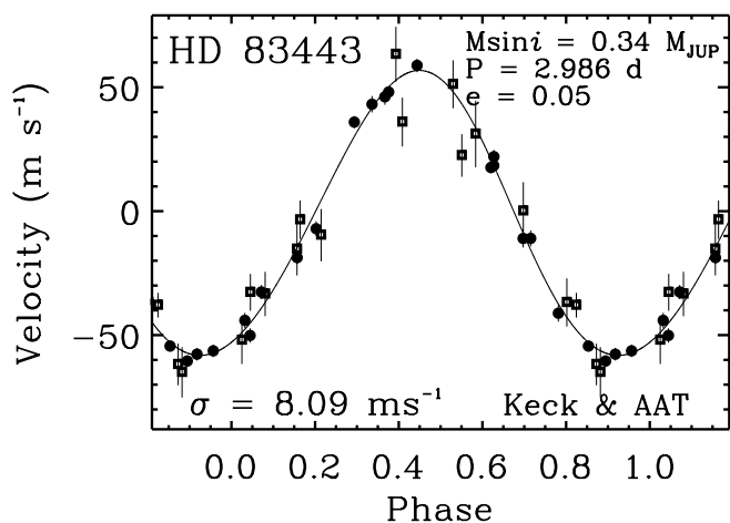
FIG. 3.—Phased Doppler velocities for HD 83443 from the combined Keck (circles) and AAT (squares) data. The solid line is the best-fit Keplerian orbit. The period p = 2.986 days and semiamplitude K = 57 \text{ m s}^{-1} are nearly identical to the CORALIE parameters for the inner planet. Within measurement uncertainty, the eccentricity derived from the Keck-AAT data set is consistent with zero, similar to other “51 Peg-like” planets.
