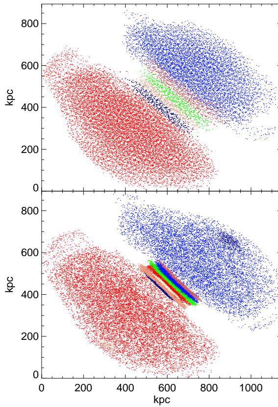
Figure 4.6: The particles of Fig. 4.5 traced back to their positions in the initial conditions. The low resolution simulation is shown in the top panel and the high resolution simulation in the bottom panel. Note the highly flattened configurations of spurious haloes.
