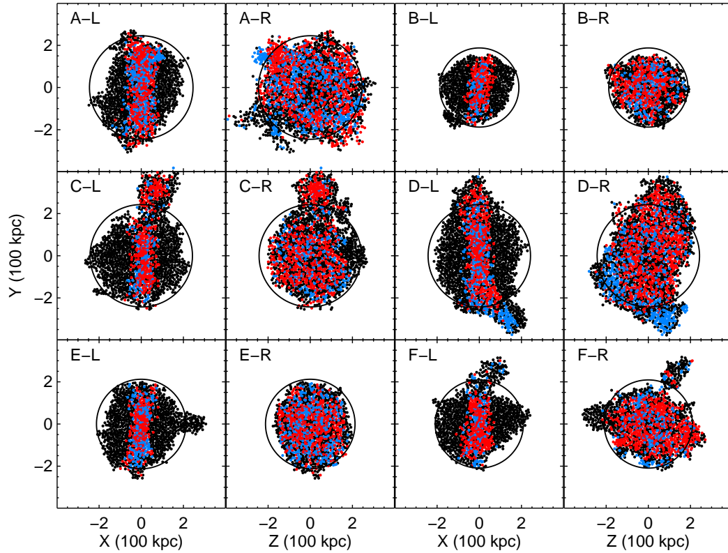
Figure 2.6: X - Y positions for subhaloes associated with the largest FOF group at z = 0 in two projections. Subhaloes with \cos \theta_{H,S} > 0.9 are indicated in red and those with \cos \theta_{H,S} < -0.9 in blue. All other subhaloes are shown in black. The black circle marks the virial radius, r_{200} . Left panels (i.e. L) : the X axis points in the direction of the main halo spin, so those subhaloes with orbit vectors parallel and antiparallel to the main halo spin appear as a band parallel to the Y axis. Right Panel (R) : looking down the X axis, so the main halo is spinning anticlockwise. The red and blue points are plotted in a random order on top of the black.
