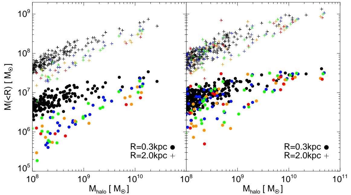
Figure 4.19: Central masses of field haloes (left) and subhaloes within r_{200b} (right), evaluated within radii of 2 kpc (crosses) and 300 pc (circles) as a function of total mass. Different colours correspond to different simulations: black for CDM-W7, blue, green, orange and red for models m_{2.3} , m_{2.0} , m_{1.6} , and m_{1.4} respectively.
