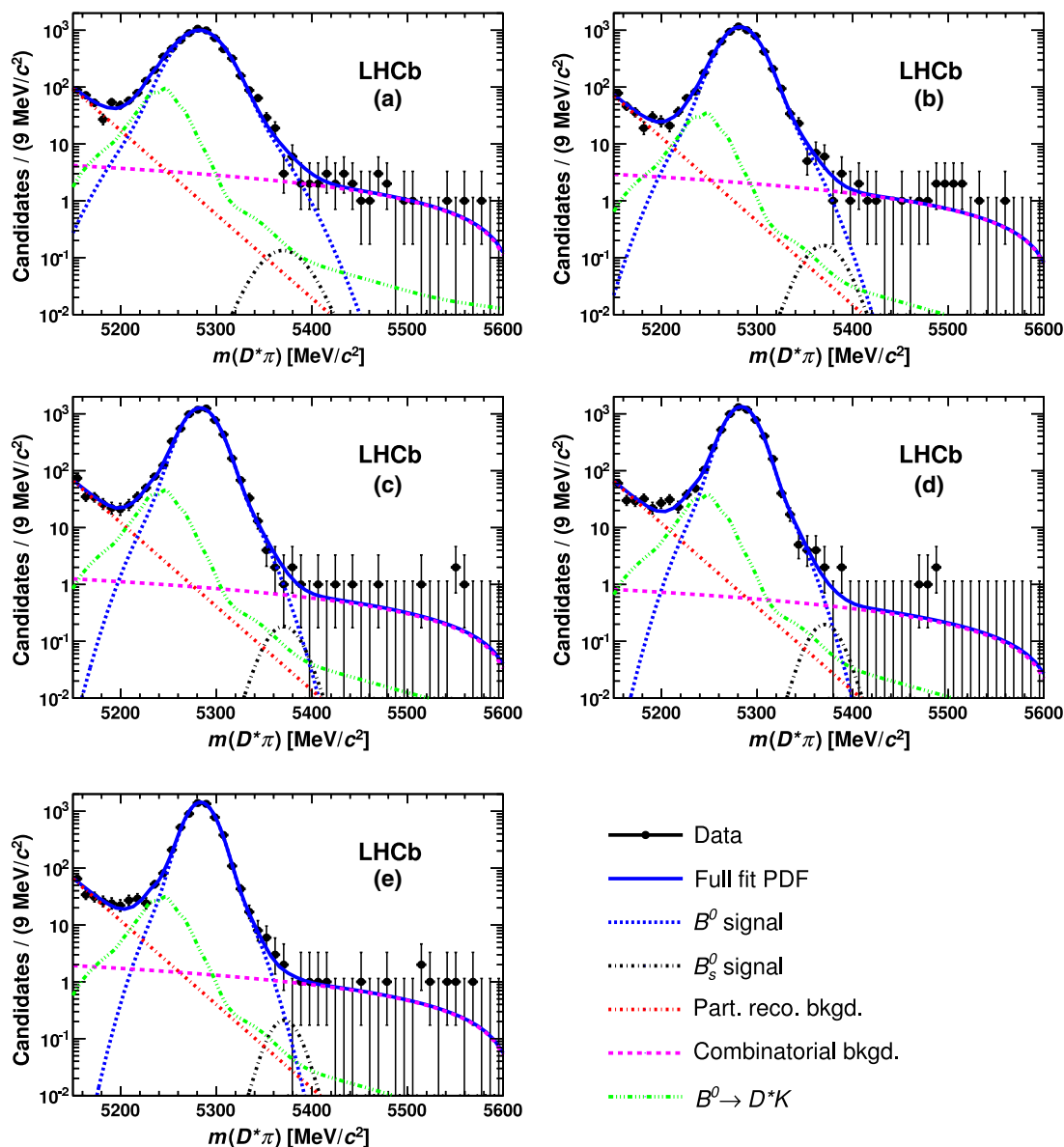
FIG. 2 (color online). Simultaneous fit to the full data sample in five bins of \theta_{\text{bach}} : (a) 0–0.046, (b) 0.046–0.067, (c) 0.067–0.092, (d) 0.092–0.128 and (e) 0.128–0.4 rad. Note the y-axis scale is logarithmic and is the same for each bin. Data points are shown in black, the full PDF as a solid blue line and the component PDFs as follows: (red dot-dashed line) partially reconstructed background, (magenta dashed line) combinatorial background, (blue dashed line) B^0 signal, (black dot-dashed line) B_s^0 signal and (green three-dot-dashed line) B^0 \rightarrow D^{*-} K^+ background.
