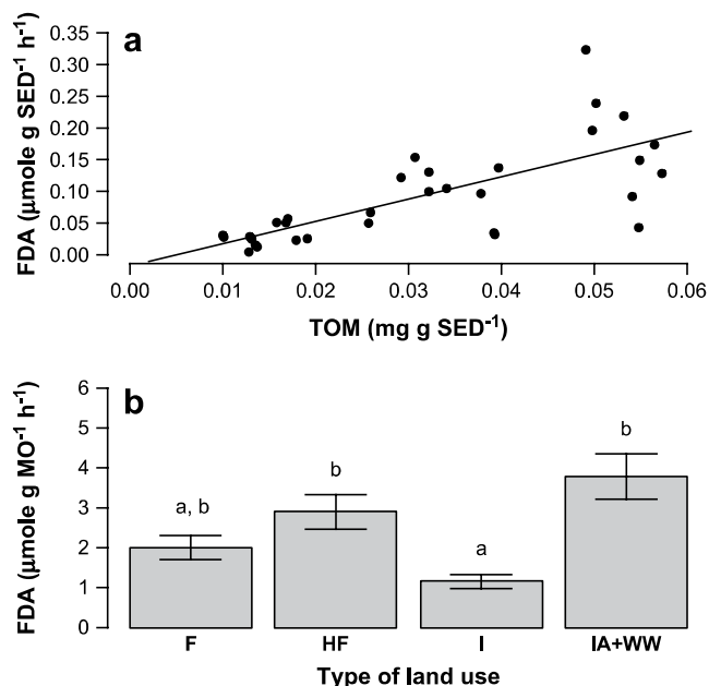
Fig. 3. (a) Relationship between hydrolasitic microbial activity (FDA hydrolysis reported per gram of dry sediment per hour) and the total organic matter content of the sediment (mg TOM per gram of dry sediment) ( R^2 = 0.51 , y = 3.34x - 0.01 , p < 3.10^{-6} ). (b) Changes in hydrolasitic microbial activity (mean \pm 95% SE, expressed in FDA hydrolysis per gram of TOM per hour) according to the four types of land use (F=Forest; HF=Hedged farmland; IA=Intensive agriculture; IA+WW=Intensive agriculture plus waste water). For each grouping, significant between-type differences (multiple comparison tests following the Kruskal–Wallis test) in hydrolasitic microbial activities are indicated by different letters.
