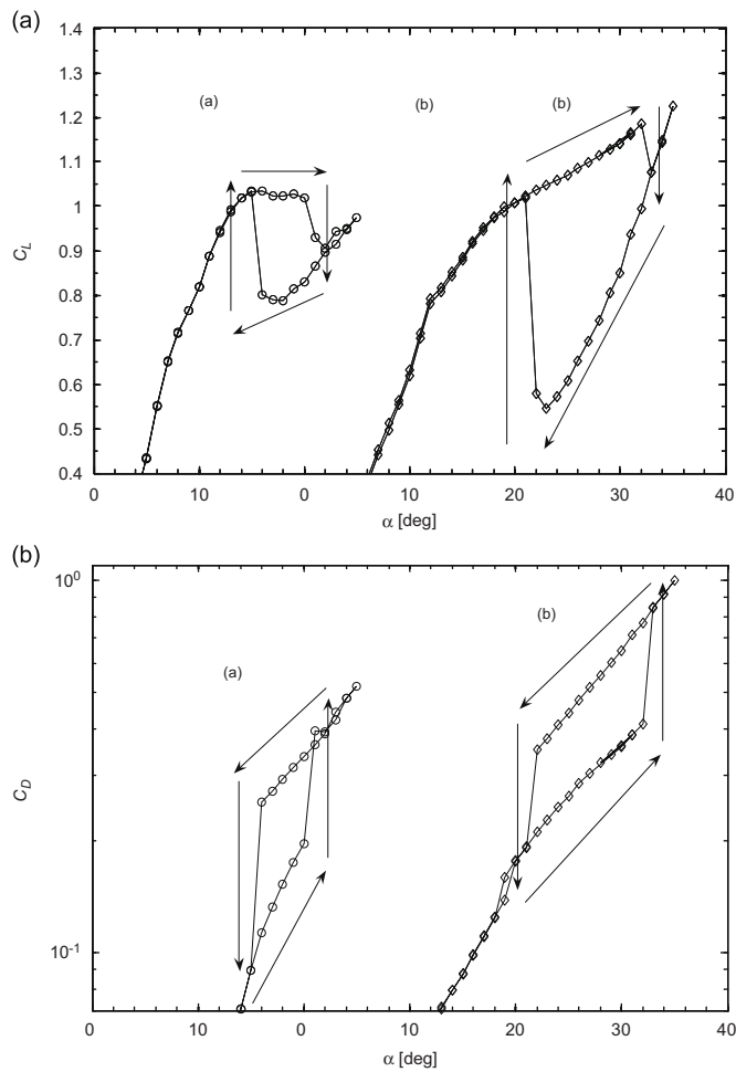
Fig. 5. (A) Close-up of the hysteric behaviour of the lift coefficients, and (B) the drag coefficients, for (a) NACA0015 and (b) NACA0025.
