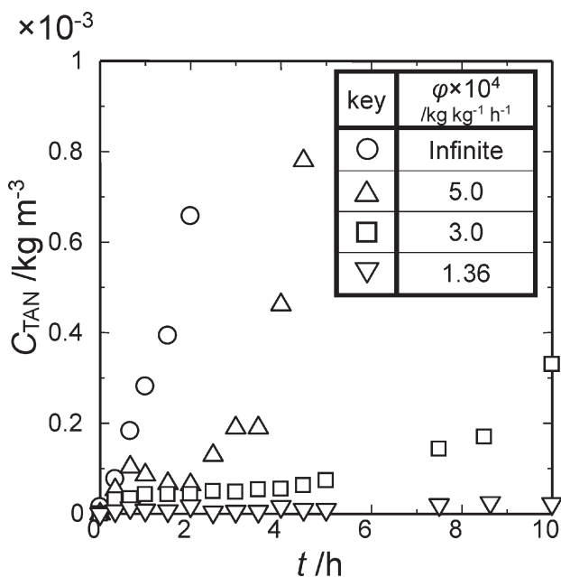
Fig. 8 – Time courses of ammonia-nitrogen concentration in culture solution for semi-continuous uptake measurements; C_{\text{in}}: 1.0 \times 10^{-3} \text{ kg m}^{-3} , V_{\text{in}}: 0\text{--}6.0 \times 10^{-4} \text{ m}^3 \text{ h}^{-1} , \rho_{u,0}: 2.4 \text{ kg m}^{-3} , T: 303 \text{ K} , \text{PFP}: 1800 \mu\text{mol m}^{-2} \text{ s}^{-1}
