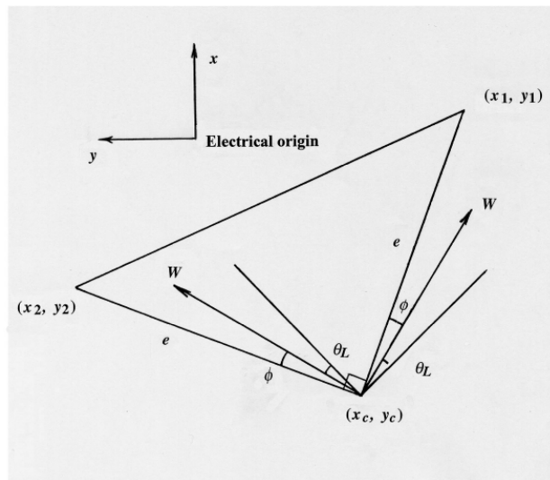
Fig 3 – Shaft centre and rotor eccentricity
