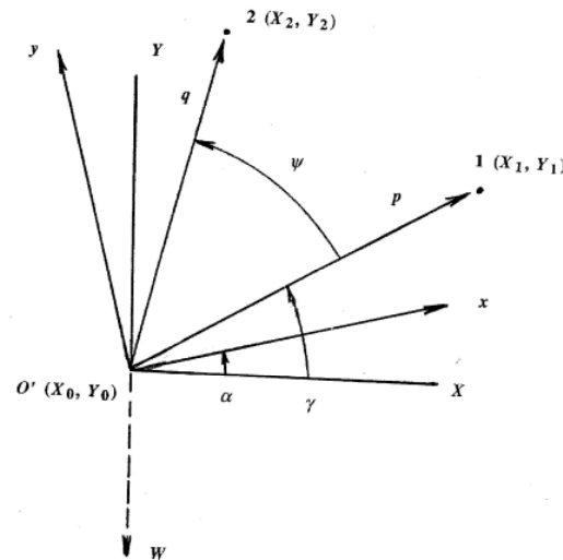
Fig 4 – Reference axis sets and angles used
