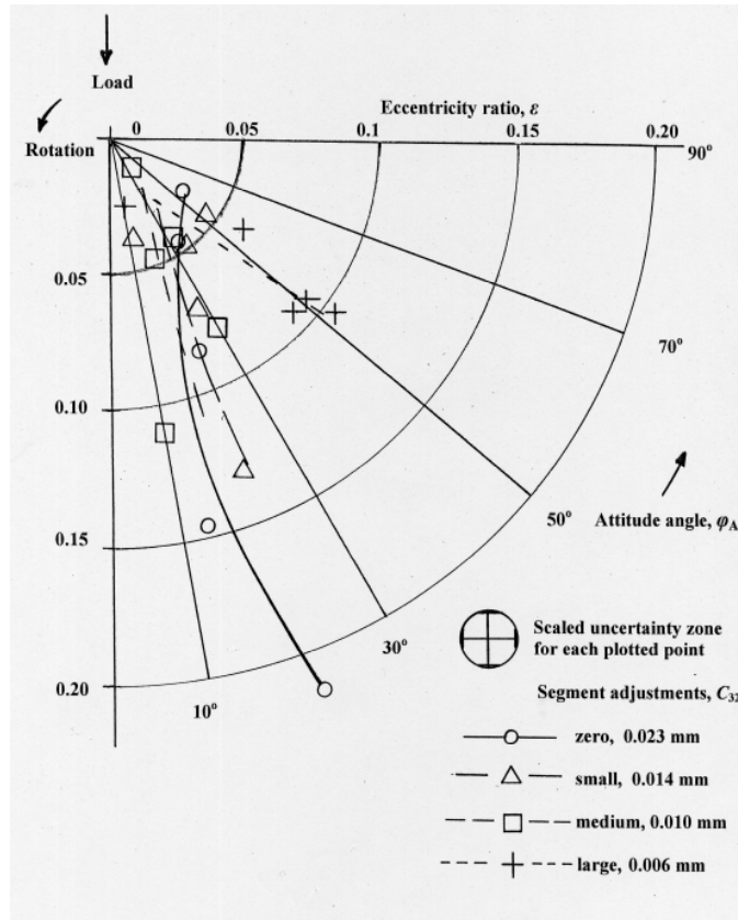
Fig 5 Static locus plots for different adjustments, 3500 rpm
