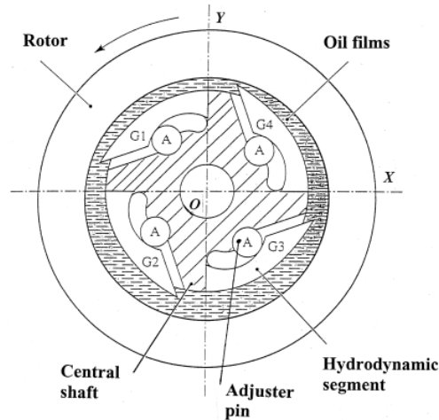
Fig 2 – Cross section scheme of adjustable hydrodynamic segments
