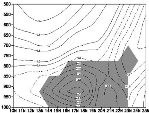
Figure 4. Latitude-height section of mean ERA-40 zonal wind ( \text{m.s}^{-1} ) composite difference anomalies along 18^\circ\text{E} for a sample of 8 high minus 8 low dust months during January–April 1979–92. Contours 0.5 \text{ m.s}^{-1} , shading shows significant differences at 0.05 level.
