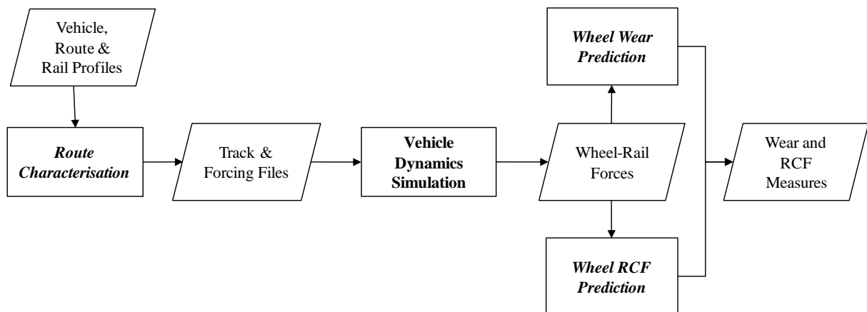
Figure 3 Methodology of the Wheel Damage Model
