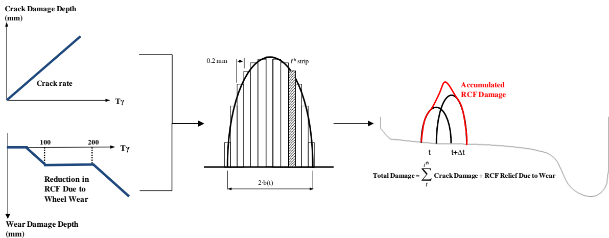
Figure 8 Methodology of RCF Damage Prediction
