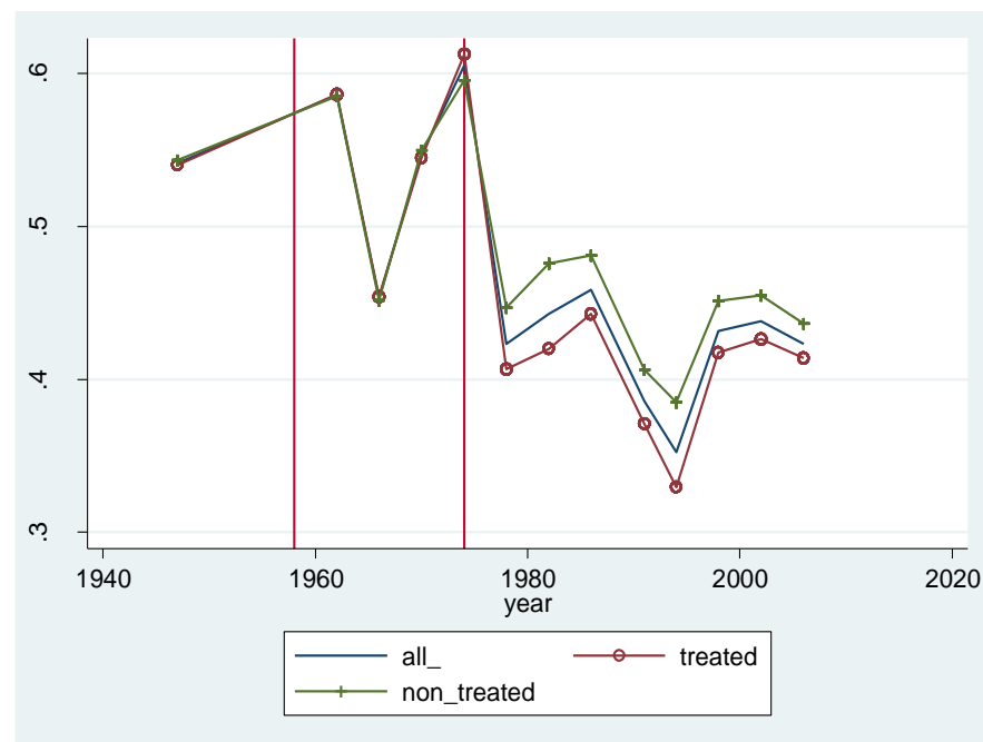
Graph 4. Mean electoral turnout among Colombian departments 1947 - 2006
