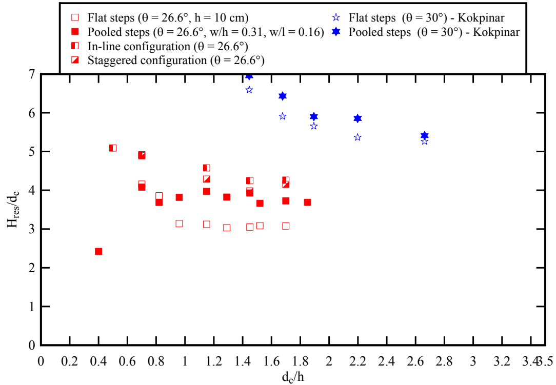
Fig. 12 - Dimensionless residual head at the downstream end of the 10-step stepped spillways - Comparison between flat stepped chute, pooled step chute, and in-line and staggered configurations of flat and pooled steps (Present study), as well as with the re-analysed data of Kökpinar (2004) - All data were estimated based upon detailed air-water flow measurements
