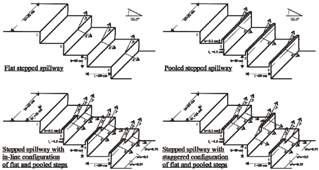
Fig. 2 - Definition sketch of the stepped configurations
