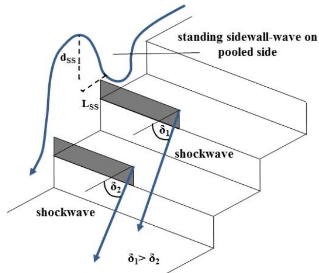
Fig. 6 - Definition sketches of sidewall standing waves and shock waves in stepped chutes with in-line and staggered configurations of flat and pooled steps
