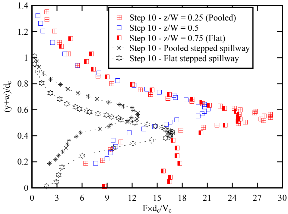
Fig. 10 - Dimensionless bubble count rate distributions on the stepped spillway with staggered configuration of flat and pooled steps in skimming flows ( \theta = 26.6^\circ ): d_c/h = 1.70 , Q = 0.113 \text{ m}^3/\text{s} , Re = 8.72 \times 10^5 - Comparison with flat and pooled stepped spillways for identical flow conditions
