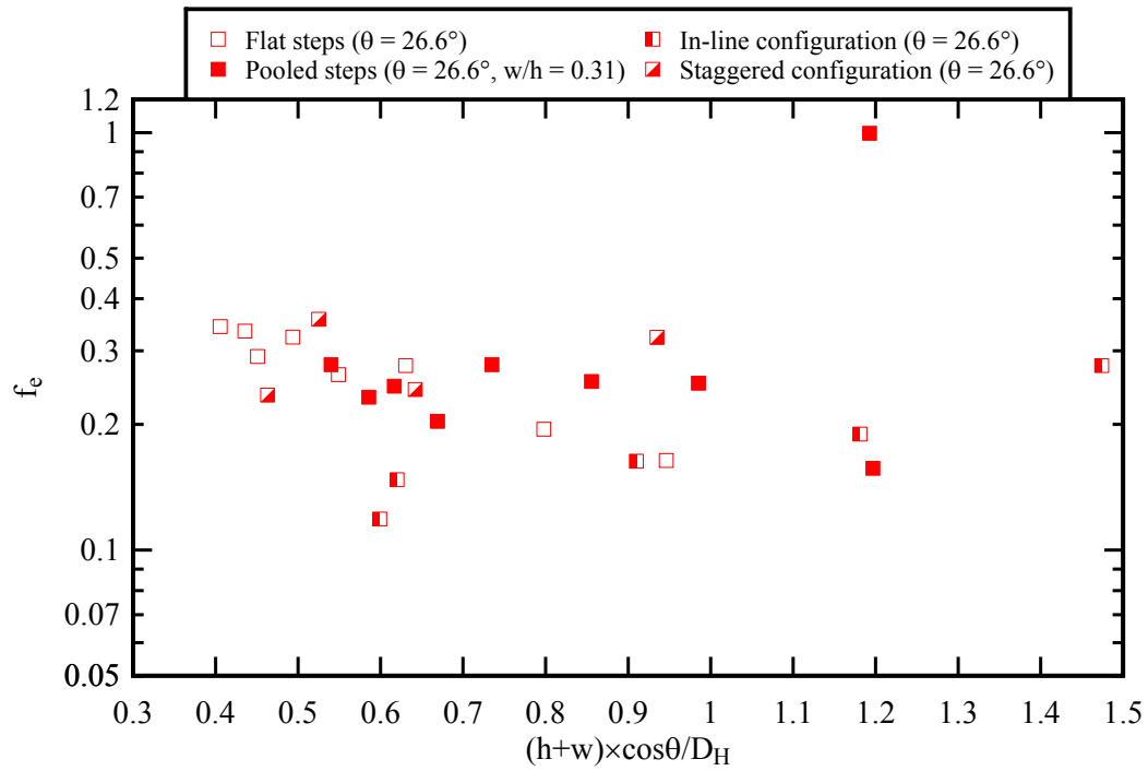
Fig. 13 - Darcy friction factors on flat and pooled stepped spillways (all four configurations) - All data were calculated based upon detailed air-water flow measurements
