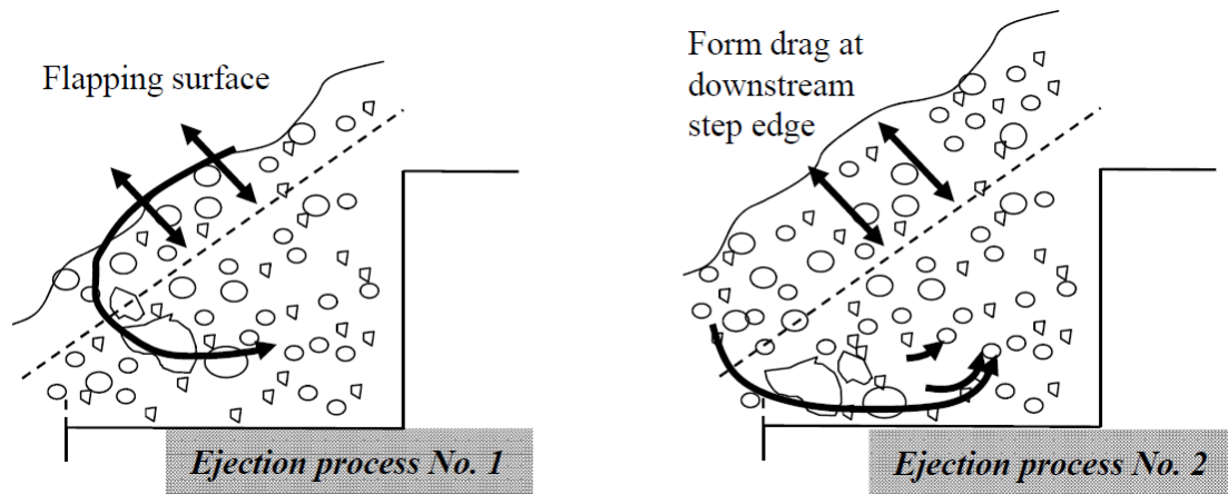
Fig. 7 - Sketch of cavity ejection processes on flat and pooled stepped spillways ( \theta = 26.6^\circ )
