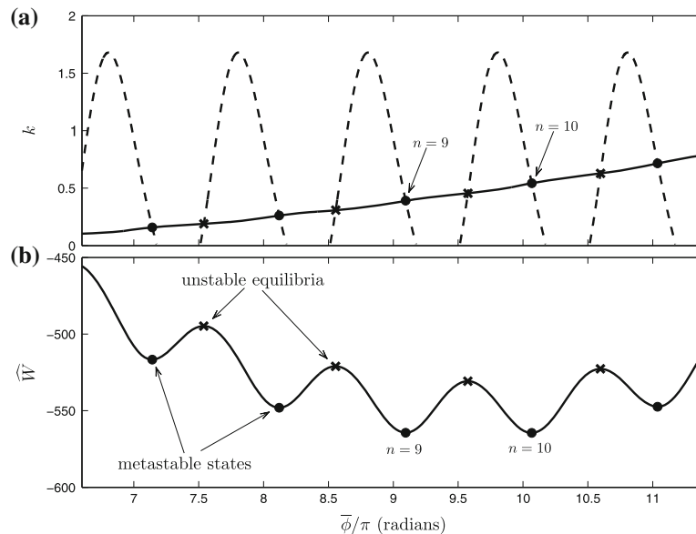
Fig. 2 a Constant of integration k derived from implicit Eq. (12) (solid line) and boundary condition (13) (dashed line) as angle \bar{\phi} varies, with \lambda = 32.58 , \rho = 0.1 , \zeta = 0 and \hat{q} = 10 . b Energy \hat{W} , where k is calculated using the implicit form (12). Intersections of k -curves coincide with energy extrema and allow us to calculate the energy profile \phi(z) via (10)
