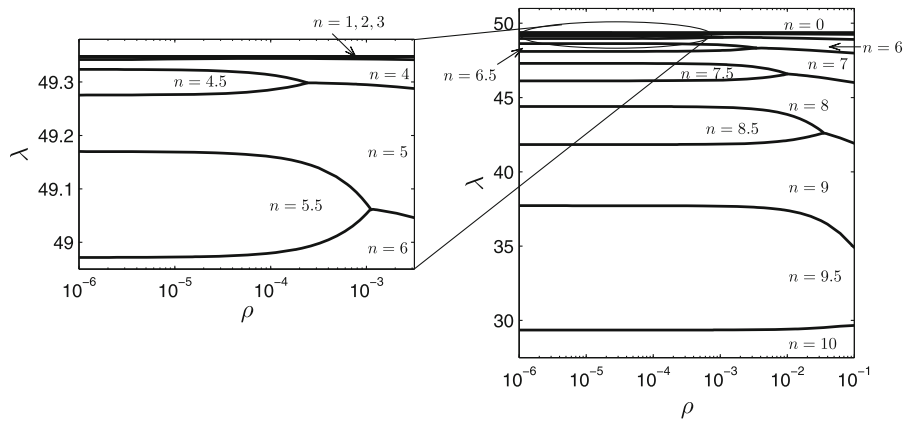
Fig. 7 Regions in (\lambda, \rho) space where different n -states act as global energy minimum for \zeta = -1, \hat{q} = 10 . The states n = 1, 2 and 3 occur in the small region before the helix unwinds but cannot be distinguished in the figure
