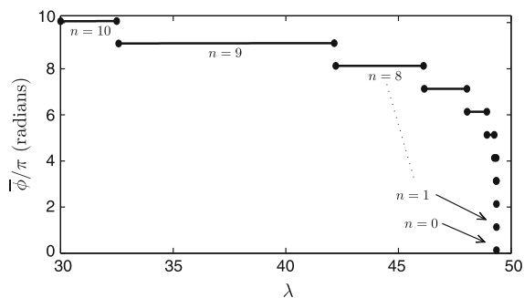
Fig. 4 Azimuthal twist angles at upper plate for variable parameter \lambda , with \rho = 0.1 , \zeta = 0 and \hat{q} = 10 . As the field strength increases, the global minimum energy state expels (approximate) half-twists and the cholesteric helix unwinds. The cascade of pitchjumps from n = 4 to n = 0 takes place over a very short interval when \lambda is large and the helix is nearly unwound. Note, as seen in Fig. 3, the twist angles at the upper surface are close but not equal to integer multiples of \pi radians because of the weak anchoring condition
