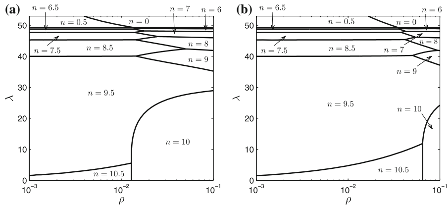
Fig. 8 Regions in (\lambda, \rho) space where different n -states are global energy minimum for \hat{q} = 10 : a \zeta = -1.01 ; b \zeta = -1.1 . As \zeta decreases, the secondary states dominate the cholesteric transition to a planar nematic
