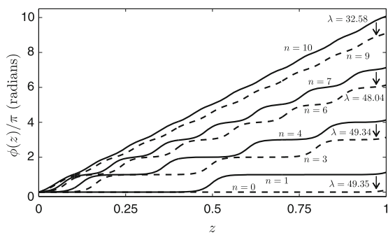
Fig. 3 Unwinding of director twist \phi(z) at specific values of parameter \lambda with \rho = 0.1 , \zeta = 0 and \hat{q} = 10 . In each case, the chosen \lambda corresponds to a critical value where the helix expels a half-twist as the cholesteric unwinds. For each profile, n represents the number of half-twists rounded to the nearest integer multiple of 0.5
