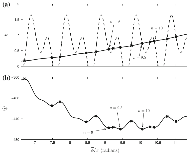
Fig. 5 a Constant of integration k derived from implicit Eq. (12) (solid line) and boundary condition (13) (dashed line) as angle \bar{\phi} varies, with \lambda = 29.50 , \rho = 0.1 , \zeta = -1 and \hat{q} = 10 . b Energy \bar{W} , where k is calculated using implicit form (12). Oscillations in k -curve obtained from (13) result in secondary metastable states
